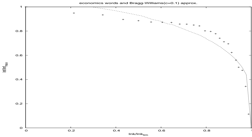
FIG. 4. Vertical axis is \frac{\ln f}{\ln f_{max}} and horizontal axis is \frac{\ln k}{\ln k_{lim}} . The + points represent the words of the economics dictionary with the fit curve being Bragg-Williams in presence of magnetic field, c = \frac{H}{\gamma\epsilon} = 0.1 .
