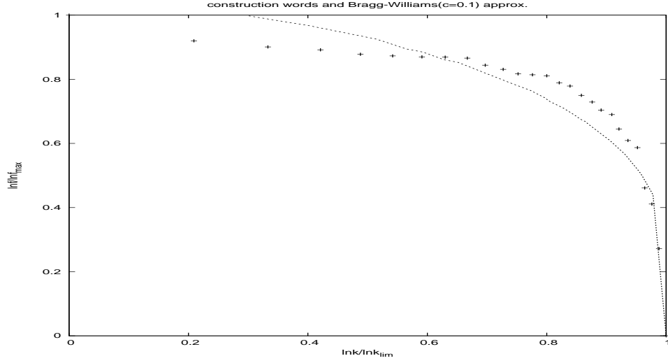
FIG. 41. Vertical axis is \frac{\ln f}{\ln f_{max}} and horizontal axis is \frac{\ln k}{\ln k_{lim}} . The + points represent the words of the dictionary of construction etc. with fit curve being Bragg-Williams curve in presence of magnetic field, c = \frac{H}{\gamma\epsilon} = 0.1 .
