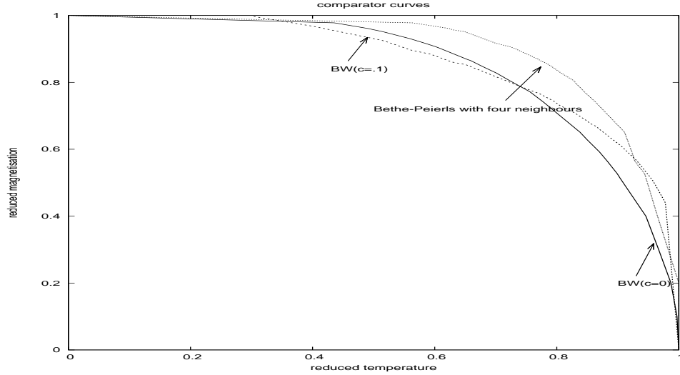
FIG. 1. Reduced magnetisation vs reduced temperature curves for Bragg-Williams approximation, in absence(dark) of and presence(inner in the top) of magnetic field, c = \frac{H}{\gamma\epsilon} = 0.1 , and Bethe-Peierls approximation in absence of magnetic field, for four nearest neighbours (outer in the top).
