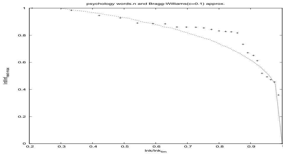
FIG. 23. Vertical axis is \frac{\ln f}{\ln f_{next-max}} and horizontal axis is \frac{\ln k}{\ln k_{lim}} . The + points represent words of the psychology dictionary with fit curve being Bragg-Williams curve in presence of magnetic field, c = \frac{H}{\gamma \epsilon} = 0.1 .
