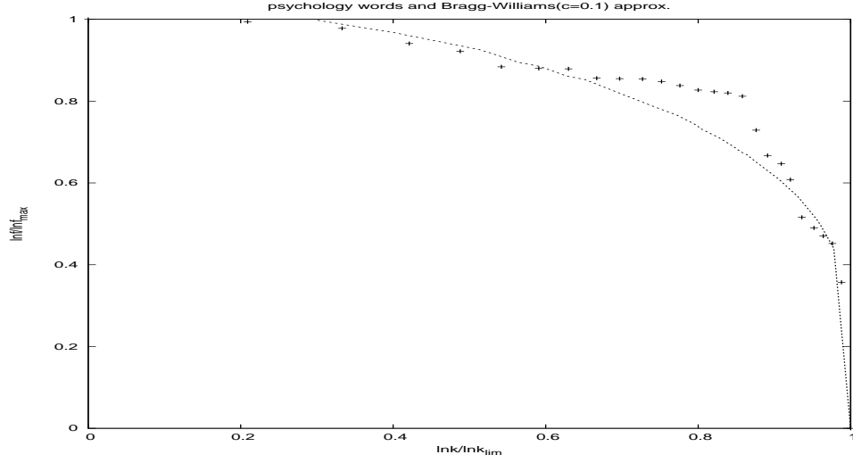
FIG. 22. Vertical axis is \frac{\ln f}{\ln f_{max}} and horizontal axis is \frac{\ln k}{\ln k_{lim}} . The + points represent words of the psychology dictionary with fit curve being Bragg-Williams curve in presence of magnetic field, c = \frac{\mu H}{\gamma J} = 0.1 .
