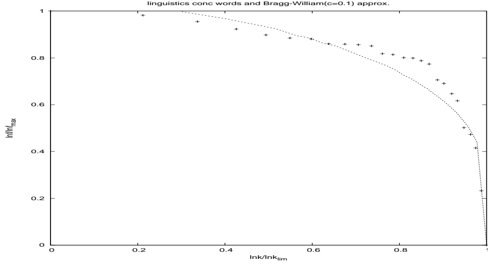
FIG. 16. Vertical axis is \frac{\ln f}{\ln f_{max}} and horizontal axis is \frac{\ln k}{\ln k_{lim}} . The + points represent the words of the linguistics dictionary with fit curve being Bragg-Williams curve with magnetic field, c = \frac{H}{\gamma\epsilon} = 0.1 .
