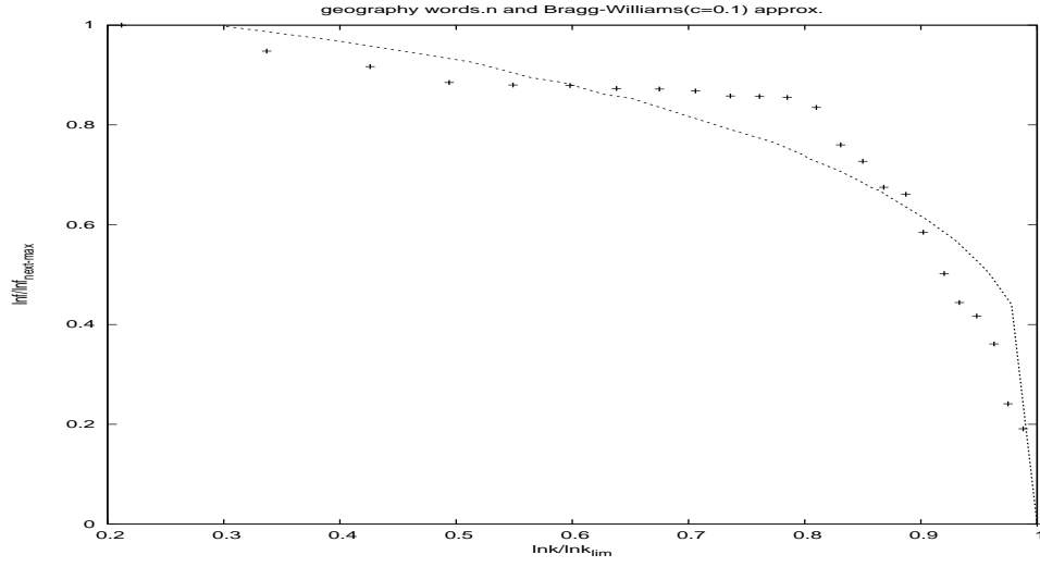
FIG. 11. Vertical axis is \frac{\ln f}{\ln f_{next-max}} and horizontal axis is \frac{\ln k}{\ln k_{lim}} . The + points represent the words of the geography dictionary with fit curve being Bragg-Williams curve in presence of magnetic field, c = \frac{H}{\gamma\epsilon} = 0.1 .
