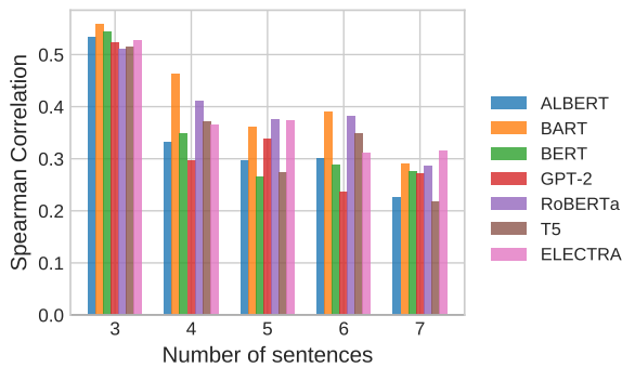
Figure 4: Sentence ordering task breakdown based on the best layer of each model.
