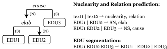
Figure 1: Illustration of the RST discourse probing tasks (Tasks 4–6).
