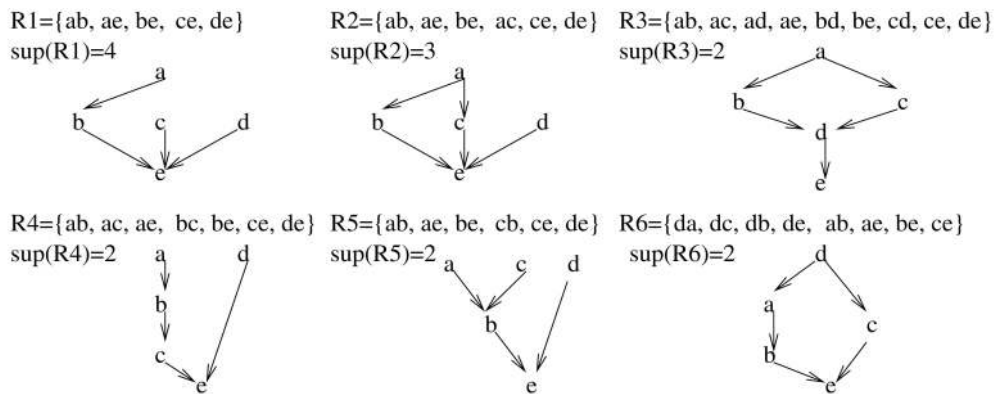
Fig. 5. The frequent closed itemsets and the transitive reductions of the corresponding frequent CPOs.
