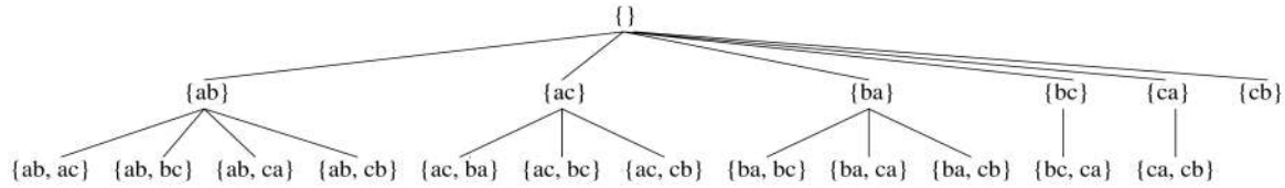
Fig. 7. The set enumeration tree of the transitive reductions of all possible partial orders on items a , b , and c .
