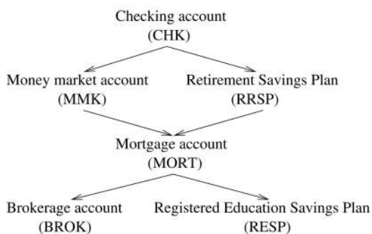
Fig. 1. A frequent partial order R in Example 1.
