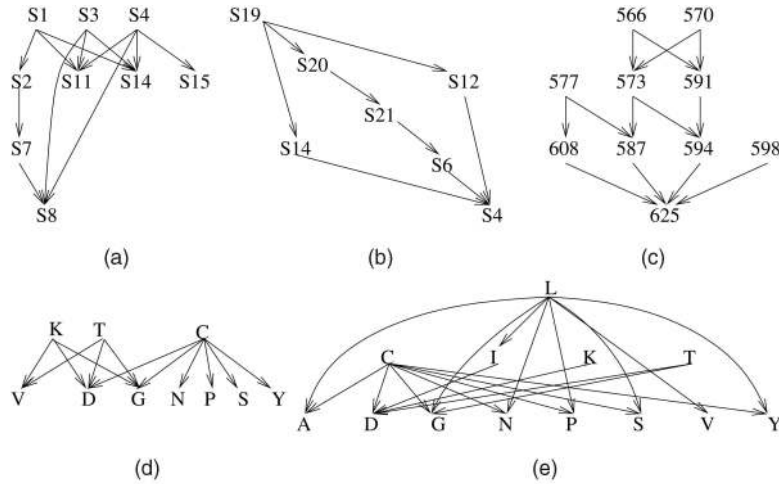
Fig. 10. Some frequent closed partial orders found in real data sets. (a) A pattern in data set Yeast (support=80). (b) A pattern in data set BreastCancer (support=224). (c) A pattern in data set Gazelle (support=10). (d) A pattern in data set Snake (support=107). (e) Another pattern in data set Snake (support=80).
