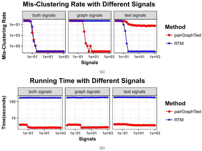
FIG. 11. Comparison between pairGraphText and RTM .
