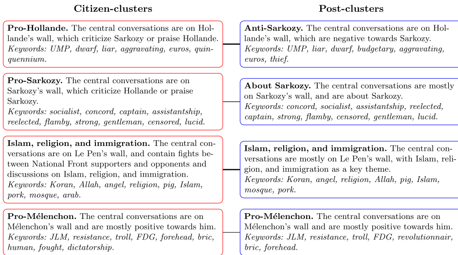
FIG. 8. Cluster topics when h = 0 .
