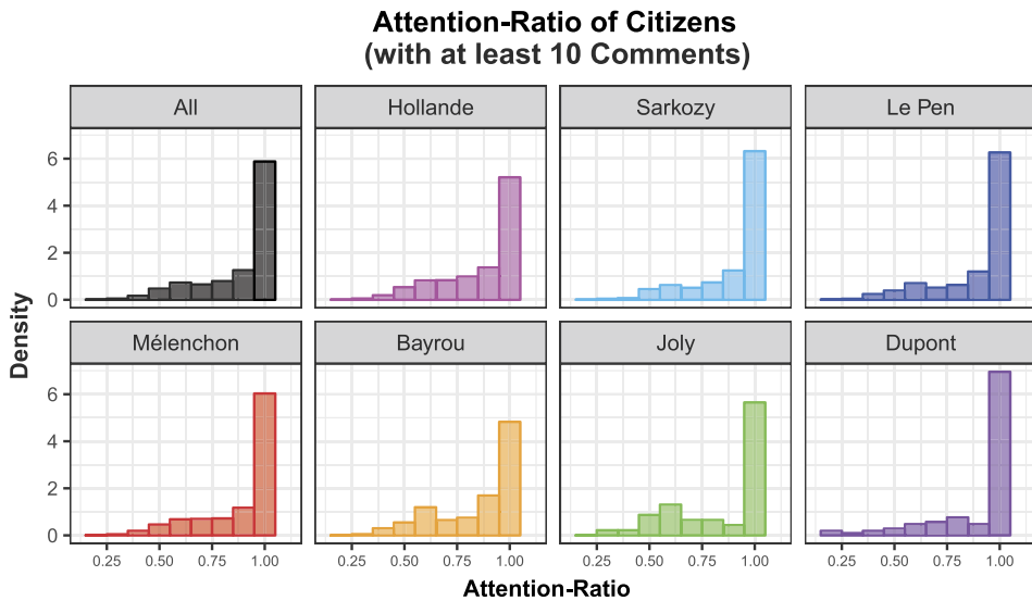
FIG. 3. Distribution of citizens’ attention-ratio. In this figure, we focus on citizens who have at least 10 comments. The first plot displays the histogram of attention-ratio for all citizens. The rest eight plots are for the eight citizen-clusters based on the candidates they focus on. We don’t display the citizens who focus on Poutou, because he attracts very few comments.
