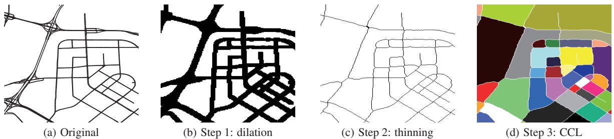
Figure 3: Map Segmentation
