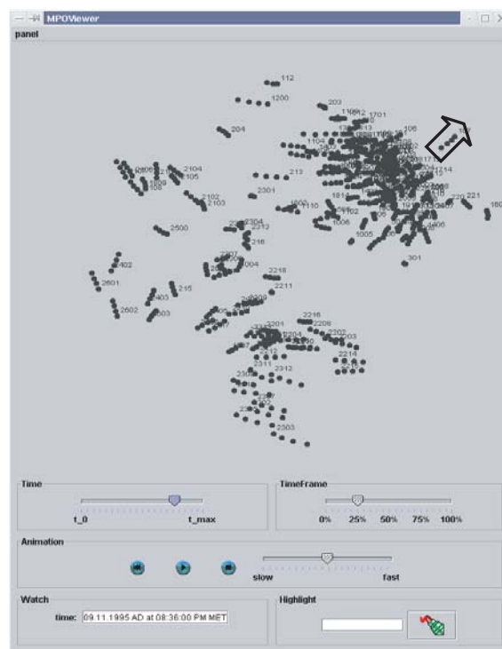
Figure 11: Swiss districts moving in ideological space
