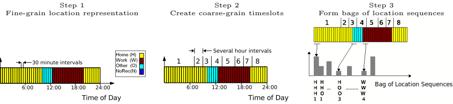
Fig. 3. The construction of the bag of location sequences explained illustratively in a 3 step process. Step 1 is the division of a day into fine-grain 30-minute time intervals, which we call the fine-grain location representation. This first step includes associating a single location label of H, W, O, or N to each 30-minute time interval. Step 2 is division of a day into 8 unevenly distributed coarse-grain time intervals. Step 3 demonstrates the word construction. Three consecutive fine-grain location labels and the coarse-grain time interval are combined to form location sequences. The set of location sequences for a day forms the bag of location sequences.
