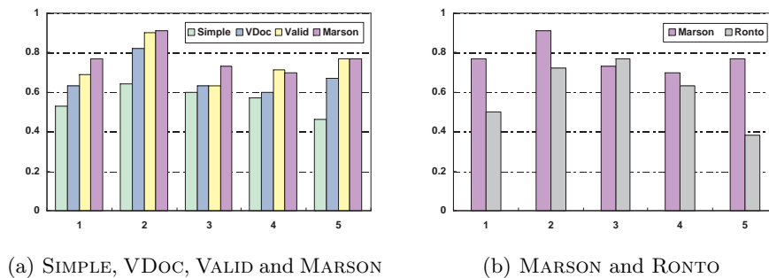
Fig. 4. Comparison of F1-Measure
