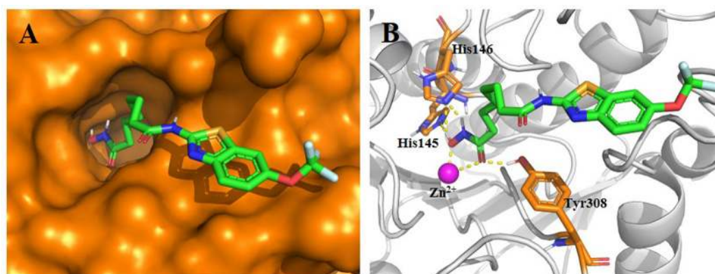
FIGURE 2 | Proposed binding mode of compound 1 (green) with HDAC2 (PDB code 4LXZ). (A) Surface of HDAC2 with compound 1 . (B) Detailed interactions between HDAC2 and compound 1 . Yellow dashed lines represent the hydrogen bonds. Oxygen, nitrogen, fluorine, sulfur, and polar hydrogen atoms are shown in red, blue, pale cyan, bright orange, and white, respectively. The Zn^{2+} is shown as a magenta sphere. The figure was generated using PyMol ( http://www.pymol.org/ ).
