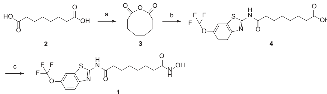
SCHEME 1 | Reagents and conditions: (a) acetic anhydride, reflux; (b) riluzole, THF, reflux; (c) ClCOO i -Bu, TEA, NH 2 OH.HCl, THF, r.t.
