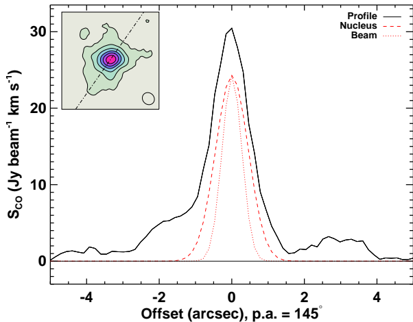
Figure 5. Slice of the CO(1–0) integrated intensity map from CARMA at a 145° position angle (see inset). The radial profile requires two Gaussians for a good fit, an “envelope” and a “nuclear” component. The nuclear component (red dashed line) has a peak intensity of 24.3 Jy beam -1 km s -1 and a FWHM of 1.05'', ( 0.82 after correcting for convolution effects from the beam). The radial profile of the beam is also shown (red dotted line), to illustrate that the nucleus is spatially resolved.
