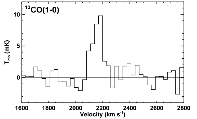
Figure 8. ^{13}\text{CO}(1-0) spectrum taken with the IRAM 30m telescope, as part of a larger census of dense gas in ATLAS ^{3\text{D}} ETGs (Crocker et al. 2011, in prep). The beam at this frequency has a 22'' half-power beam width (HPBW) and the channels shown are 30 km s ^{-1} .
