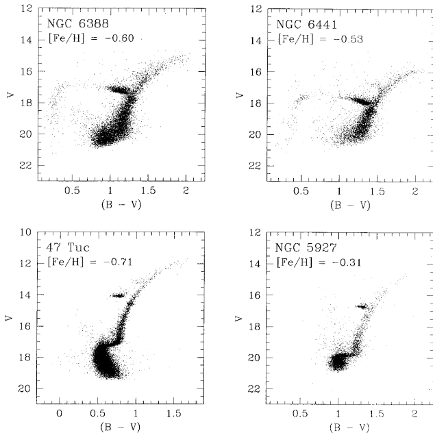
FIG. 1.—Color-magnitude diagrams constructed from F439W ( B ) and F555W ( V ) WFPC2 images of the globular clusters in this study. The red stubby horizontal branches of 47 Tuc and NGC 5927 are typical for clusters of such high metallicity ( [\text{Fe}/\text{H}] > -0.8 ). Extended blue horizontal branches (such as those in NGC 6388 and 6441) have never before been seen in such metal-rich globular clusters; they are the only two cases now known. Notice also that the morphology of the red horizontal branches of NGC 6388 and 6441 is unusual compared to the other clusters.
