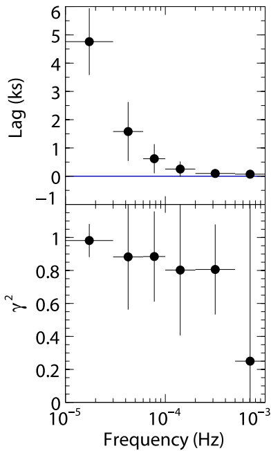
Figure 6. Lag (top) and coherence (bottom) as a function of Fourier frequency between the 4–5 and 6–7 keV energy bands for NGC 7314.
