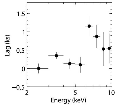
Figure 7. Energy-dependent lag for NGC 7314 at frequency of (1\text{--}30) \times 10^{-5} Hz. The whole 2–10 keV band is used as a reference.
