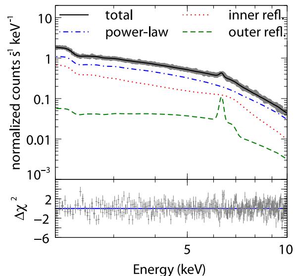
Figure 5. Best-fitting spectral model for MCG–5–23–16. The model includes a power-law component (blue dash-dotted line), outer reflection (green dashed line) modeled with reflionx , and a relativistically broadened inner reflection (red dotted line) modeled with kdblur*reflionx .
