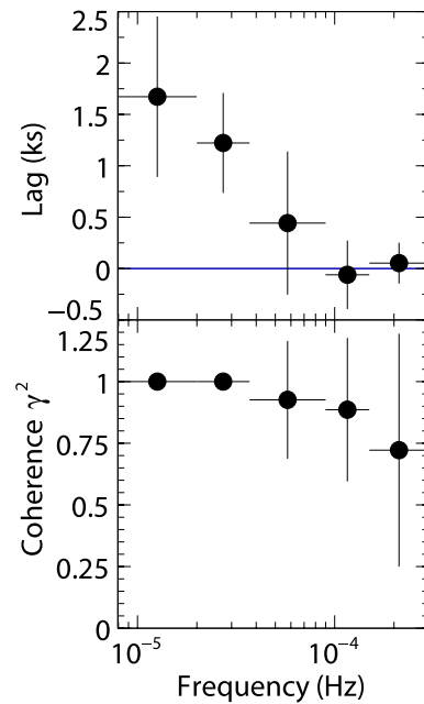
Figure 2. Lag (top) and coherence (bottom) as a function of Fourier frequency between the 4–5 and 6–7 keV energy bands for MCG-5-23-16. Positive lags in the top panel indicate hard lags, where the harder band (6–7 keV, where the reflected iron K line peaks) lags the softer band (4–5 keV, dominated by the direct emission). There is a significant hard lag at frequencies < 10^{-4} Hz. The measured coherence remains high at those frequencies.
