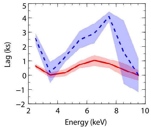
Figure 4. Lag as a function of energy for frequencies <10^{-4} (red; continuous line) and <2 \times 10^{-5} (blue; dashed line) for MCG–5–23–16. The probability that the two lines have different peaks is 85%.
