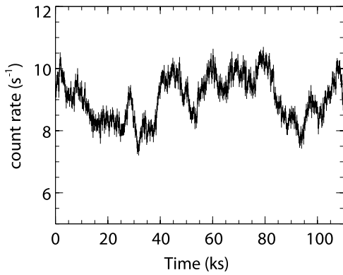
Figure 1. Light curve of MCG-5-23-16 in the 2–10 energy band. It shows the high count rate and strong variability.
