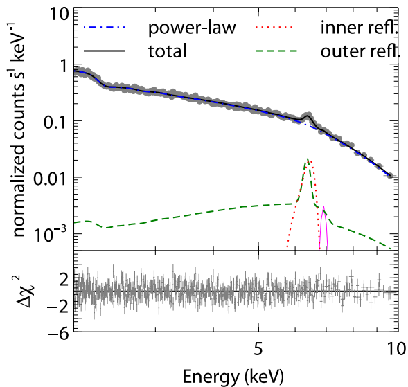
Figure 8. Best-fitting spectral model for NGC 7314. The model includes a power-law component (blue dash-dotted line), outer reflection (green dashed line) modeled with reflectionx (setting the ionization parameter to the lowest possible value of 1), and an inner reflection (red dotted line), modeled with laor and a narrow Fe XXVI line.
