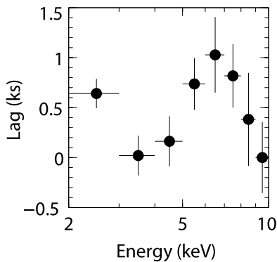
Figure 3. Lag as a function of energy for frequencies <10^{-4} for MCG–5–23–16. Energy bins have a width of 1 keV. The lags are measured with respect to a reference band taken to be the whole 2–10 keV band (see the text for details).
