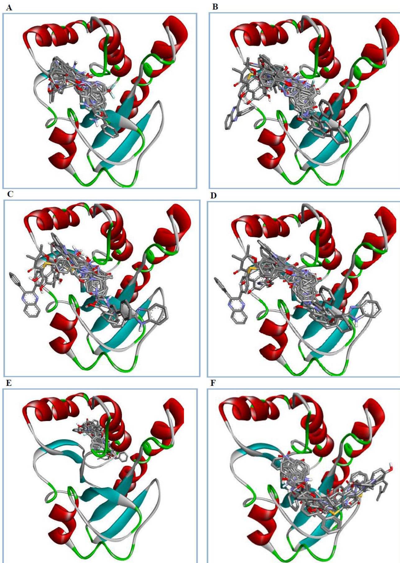
Figure S1. Structure of nsP3 with location of three binding sites at the different virtual screenings: (A) VST1; (B) VST2; (C) VST3; (D) VST4; (E) VST5; (F) VST6.
