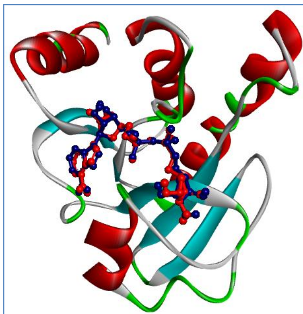
Figure 2. Superimposition of the ADP-ribose after docking (in red, the top pose) on its structure in the co-crystal structure (in blue) at the active site of nsP3. The heavy-atom RMSD between them is about 0.6 Å.
