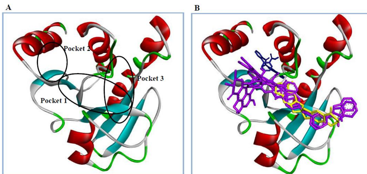
Figure 3. Representation of three binding pockets identified in the nsP3: (A) The location of three pockets in the nsP3. (B) Illustration of three pockets showing the locations of five top-hit compounds obtained from virtual screenings at these binding sites: NCI_25457, NCI_345647_a, NCI_61610 (in magenta) at the pocket 1, NCI_127133 (in blue) at the pocket 2 and NCI_670283 (in yellow) at the pocket 3.
