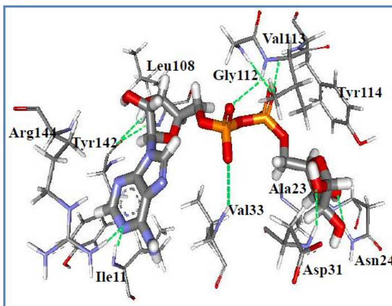
Figure 1. Re-docking ADP-ribose into the active site of nsP3: (A) The best docking pose of ligand ADP-ribose is represented as a stick model (colored by atom type) while the protein nsP3 is shown in the solvent surface (colored by interpolated charge with a probe radius of 1.4 Å). (B) The interactions of this pose and nsP3 residues showing hydrogen bonding interactions at the binding site of nsP3.
