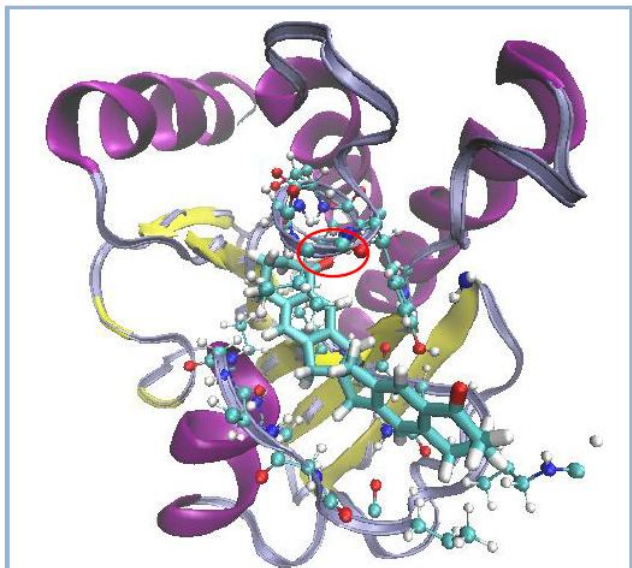
Figure 8. Hydrogen-bonding interactions between nsP3 and NCI_61610 and NCI_670283: (A) The complex of nsP3 with ligand NCI_61610 involves three strong H-bonds with residues Asn24, Tyr114 and Gly112. (B) The complex of nsP3 with ligand NCI_670283 involves one strong H-bond with Thr111 and one moderately strong H-bond with Gly112.
