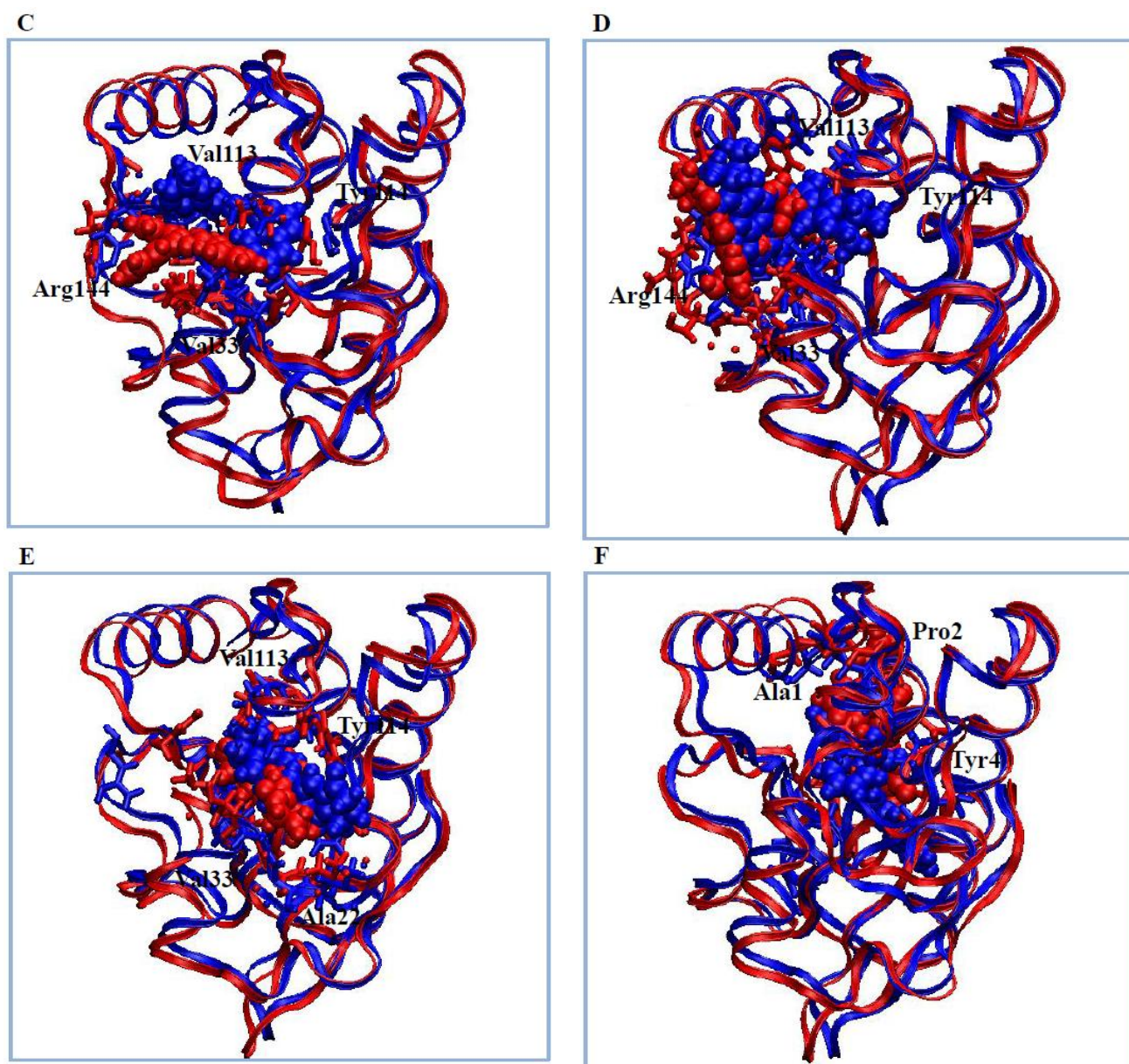
Figure 7. Superimposition of complex structures observed at 0 ns (in blue) and 23 ns (in red) with the structures represented as ribbons, the ligands as van der Waals surfaces, and the residues surrounding the ligands as sticks: (A) Apoprotein nsP3. (B)-(F): Complexes of nsP3 with the ligands NCI_61610 (B), NCI_25457 (C), NCI_345647_a (D), NCI_670283 (E), and NCI_127133 (F).
