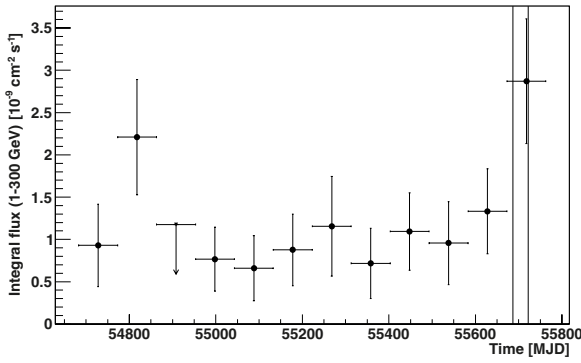
Fig. 4. Light curve with a binning of three months of the Fermi -LAT data between 1 GeV and 300 GeV. The downward pointing arrows correspond to a 95% upper limit. The vertical lines indicate beginning and end of the MAGIC observing window in 2011. The emission is consistent with a constant flux, although a trend towards a higher flux in the last bin, partially coincident with the MAGIC observations, is evident.
