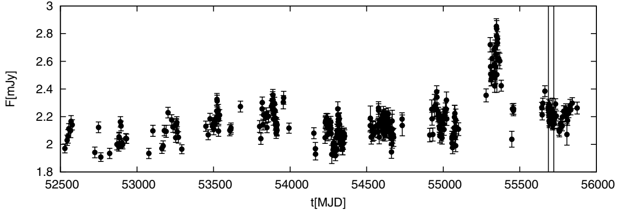
Fig. 3. Ten years light curve in the optical R -band from the Tuorla blazar monitoring program. The contribution of the host galaxy ( 1.25 \pm 0.06 mJy) has not been subtracted. Vertical lines indicate beginning and end of the MAGIC observing window in 2011. See text for details.
