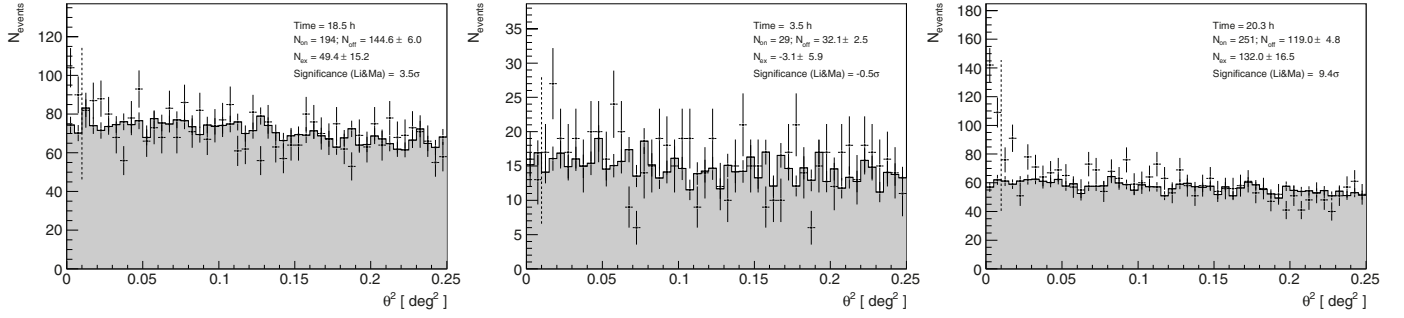
Fig. 1. Distributions of the \theta^2 parameter for 1ES 1215+303 signal (black histograms) and background estimation (gray histograms) for the three observation periods: January–February 2010 ( left ), May–June 2010 ( middle ), and January–February 2011 ( right ). The vertical dashed line corresponds to the a priori defined signal region \theta^2 < 0.01 \text{ deg}^2 .
