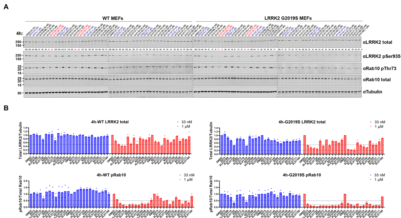
Figure 4. Screening of the second-generation PROTACs in WT and G2019S LRRK2 MEFs. (A) Representative Western blots monitoring the total LRRK2, LRRK2-pSer935, Rab10-pThr73, total Rab10, and tubulin levels after treating WT and G2019S MEFs with the indicated compounds at 33 nM, 1 \mu M, or DMSO for 4 h. (B) Quantitative analysis of the relative LRRK2 and Rab10-pThr73 levels, which are presented as ratios of total LRRK2/tubulin or Rab10-pThr73/total Rab10, normalized to the DMSO-treated sample. Data were obtained from two biological independent experiments.
