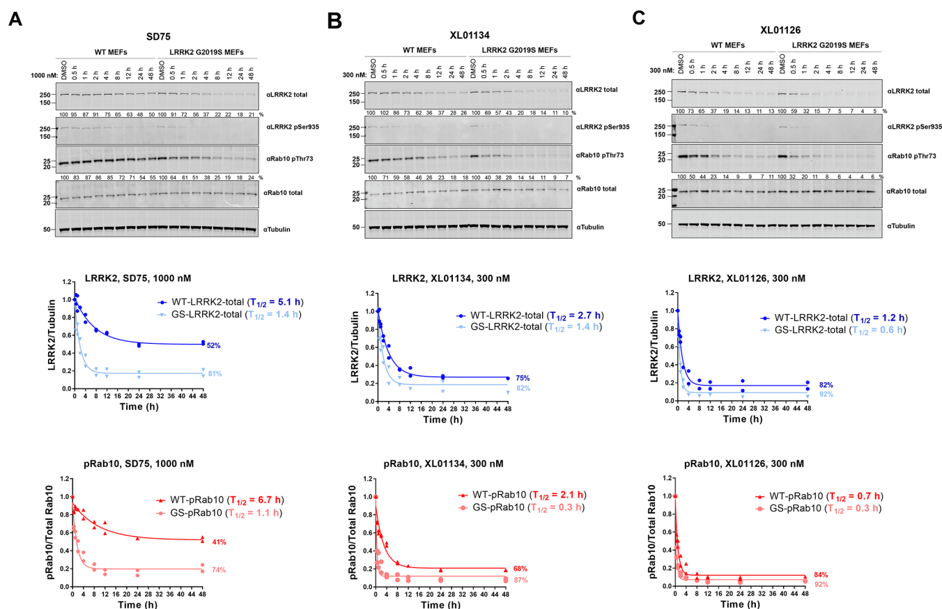
Figure 6. Time-dependent LRRK2 degradation, LRRK2 dephosphorylation, and pRab10 dephosphorylation by SD75, XL01134, and XL01126. Representative Western blots of total LRRK2, LRRK2-pSer935, Rab10-pThr73, Rab10 total, and tubulin levels after treating the WT and G2019S LRRK2 MEFs with SD75 (A), XL01134 (B), or XL01126 (C) at the indicated concentrations for the indicated period of time. The relative LRRK2 protein and pRab10 levels were obtained by quantifying the ratios of total LRRK2/tubulin or Rab10-pThr73/total Rab10, respectively, and the ratios were normalized to the DMSO-treated samples. The relative LRRK2 and pRab10 protein levels were plotted against the treatment time and were fitted against “nonlinear regression, one-phase decay” in GraphPad to obtain the half-life ( T_{1/2} ) values. Data were obtained from two independent biological experiments.
