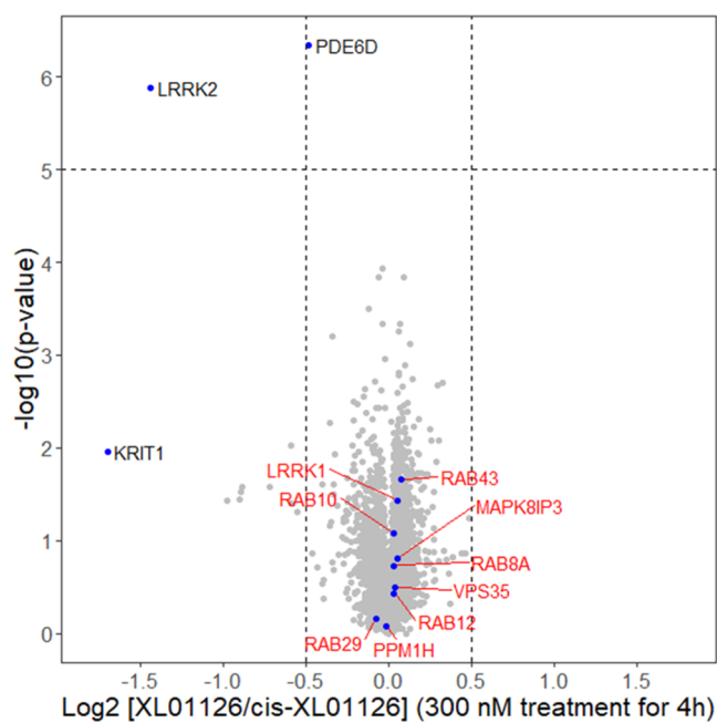
Figure 11. XL01126 induced selective LRRK2 degradation. WT MEFs were treated with 300 nM XL01126, cis -XL01126, or DMSO for 4 h and lysed (three to four replicates per condition). The lysate samples were analyzed with quantitative proteomics. Data plotted log 2 of the fold change vs cis -XL01126 control against -\log_{10} of the P value per protein. Both XL01126- and cis -XL01126-treated samples were normalized to DMSO samples before taking the ratio.
