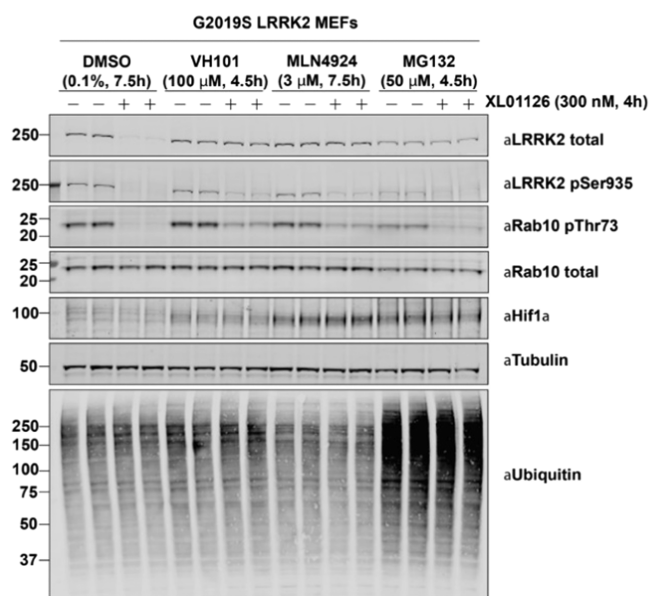
Figure 12. XL01126-induced LRRK2 degradation is rescued by VH101, MLN4924, and MG132 pretreatments. Representative Western blots of total LRRK2, LRRK2-pSer935, pRab10, total Rab10, HIF-1 \alpha , tubulin, and ubiquitinated protein after treating the G2019S LRRK2 MEFs with 300 nM XL01126 for 4 h with or without VH101, MLN4924, and MG132 pretreatments.
