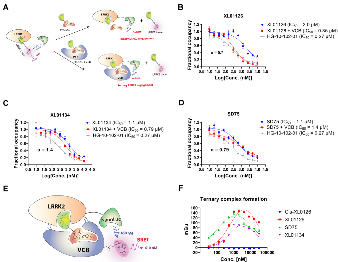
Figure 10. Binary/ternary binding affinity, cooperativity, and ternary complex formation of XL01126, XL01134, and SD75. (A). Schematic illustration of the binary and ternary LRRK2 engagement assays. HG-10-102-01, XL01126 (B), XL01134 (C), and SD75 (D) were titrated into the lysate of HEK293 cells (transfected LRRK2-NanoLuc) alone (blue line) or preincubated with VCB (red line) in the presence of LRRK2 tracer. The fractional occupancy of the tracer is plotted against the concentrations of the compounds and fitted into the “nonlinear regression, one site-log IC_{50} ” model in GraphPad to obtain the IC_{50} values. The IC_{50} ratio between the blue curve and red curve is calculated as cooperativity ( \alpha ). (E) Schematic illustration of the ternary complex formation assay (F). cis -XL01126, XL01126, SD75, and XL01134 were titrated into the lysate of HEK293 cells (transfected with LRRK2-NanoLuc) and 0.5 \mu M VCB protein labeled with Bodipy 576/589 . The NanoBRET signal was plotted against the compounds’ concentrations and fitted into “nonlinear regression, Gaussian” model in GraphPad. Error bars are mean \pm SEM from three biological independent experiments.
