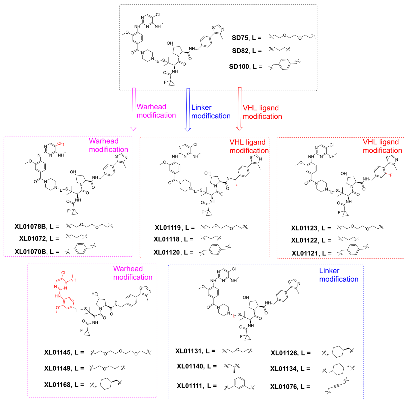
Figure 3. Second generation of LRRK2 PROTAC degraders derived from SD75, SD82, and SD100.
