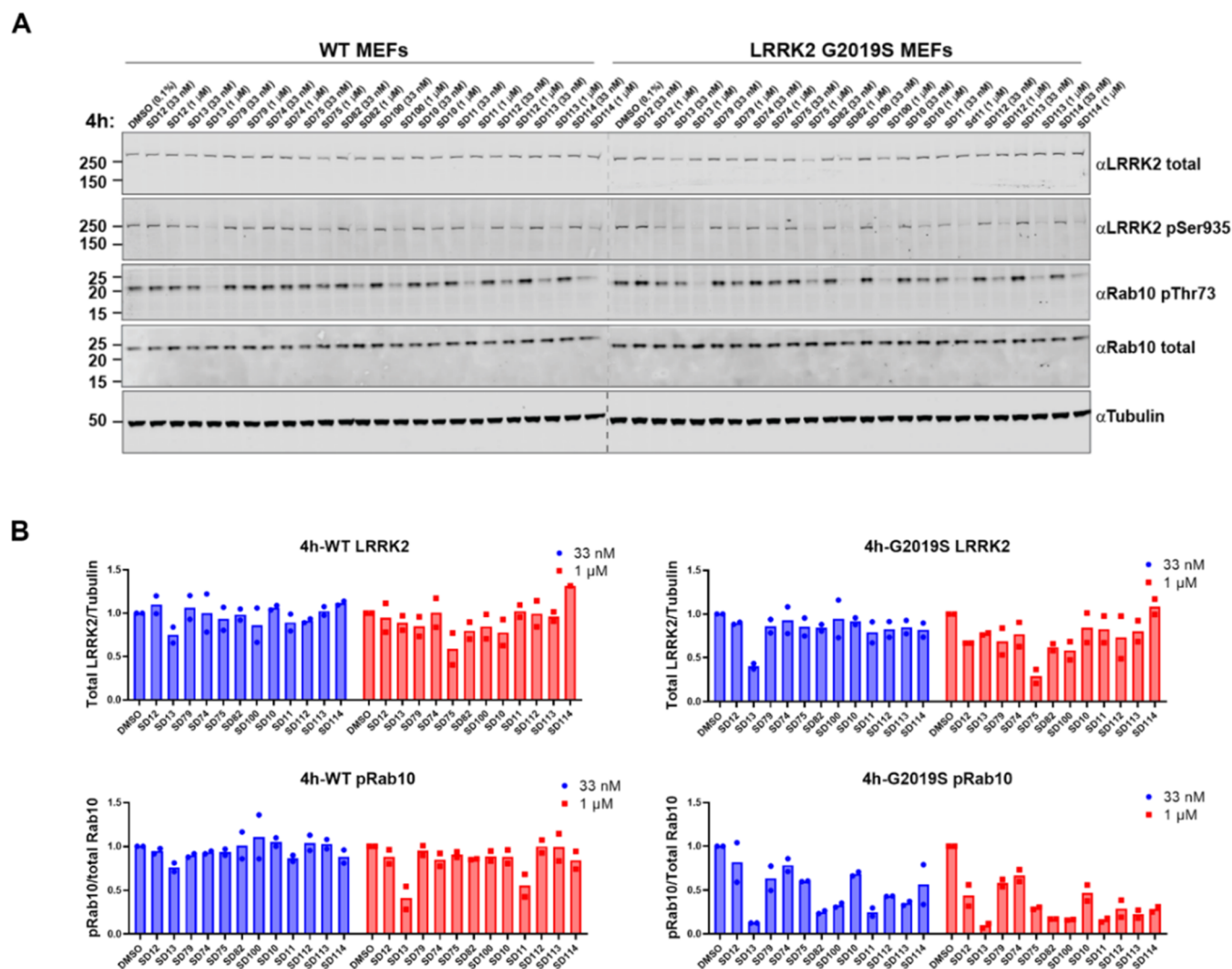
Figure 2. Screening of the first-generation PROTACs in wild-type (WT) and G2019S LRRK2 MEFs. (A) Representative Western blots monitoring the total LRRK2, LRRK2-pSer935, Rab10-pThr73, total Rab10, and tubulin levels following the treatment of WT and G2019S MEFs with the indicated compounds at 33 nM, 1 \mu M, or dimethyl sulfoxide (DMSO) for 4 h. (B) Quantitative analysis of the relative LRRK2 protein and Rab10-pThr73 levels, which are presented as ratios of total LRRK2/tubulin or Rab10-pThr73/total Rab10, normalized to the DMSO-treated sample. Data were obtained from two biological independent experiments.
