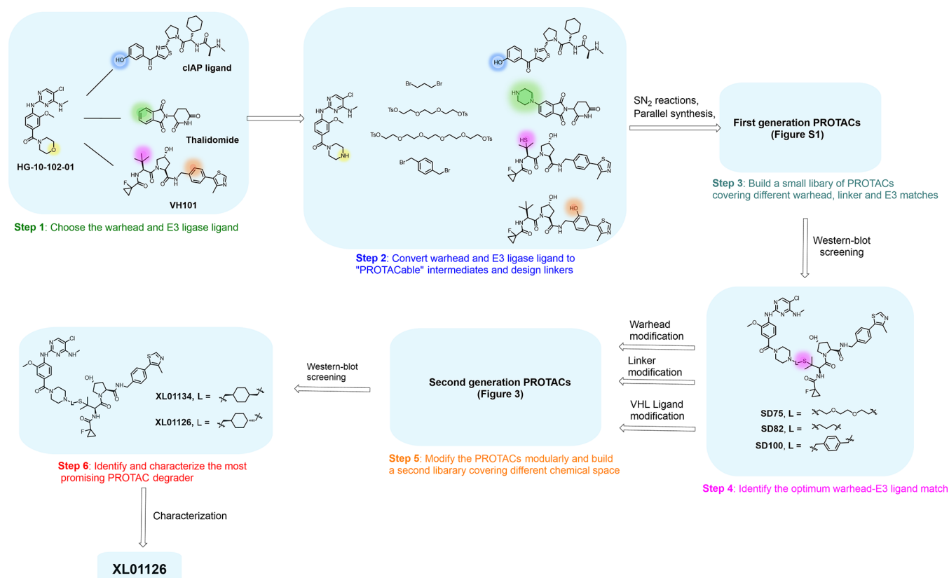
Figure 1. Our step-by-step PROTAC discovery strategies.
