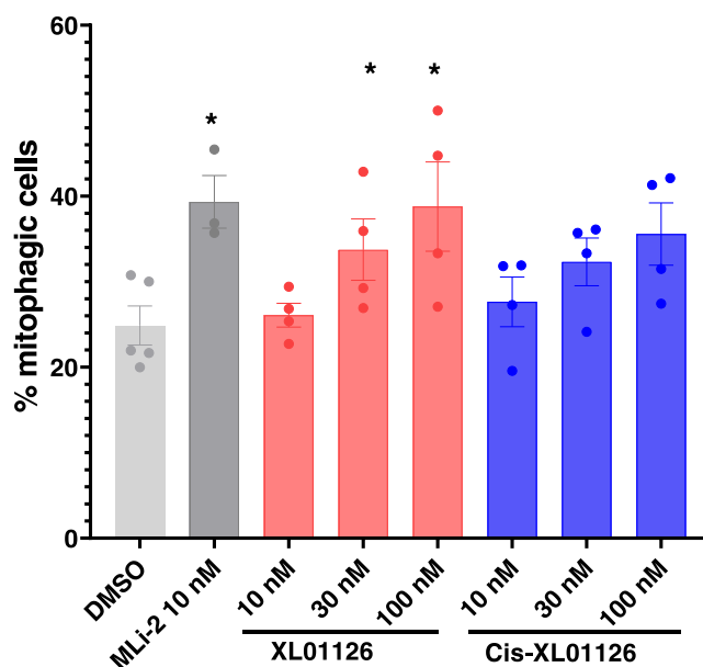
Figure 13. Effects of XL01126 and cis -XL01126 on mitophagy in Mito-QC MEFs. Quantitation of the percentage of mitophagic cells in Mito-QC MEFs after 24 h treatment with DMSO, MLI-2, XL01126, or cis -XL01126 at the indicated concentrations. Data are represented as mean \pm SEM from three to five independent experiments. Statistical significance is displayed as * p < 0.05 compared with the DMSO-treated sample.
