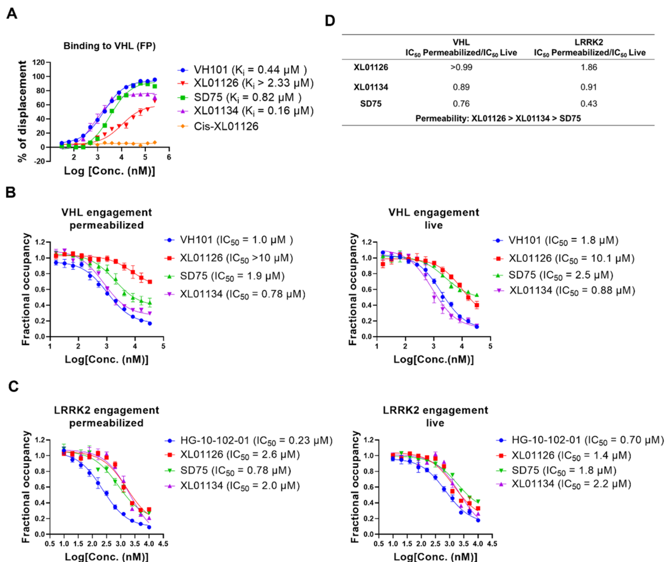
Figure 9. Binding affinities to VHL and LRRK2. (A) Binding affinity of the tested compounds to VHL using the FP assay. The indicated compounds were titrated to a solution of VCB protein (10 nM) and JC9 (5 nM) (a FAM-labeled probe that binds to VCB) to displace JC9, and the percentage of displacement was plotted against the compounds' concentration and fitted into the "nonlinear regression, one site-log \text{IC}_{50} " to obtain the \text{IC}_{50} values, which were used to back-calculate the K_i values. NanoBRET target engagement assays of tested compounds to VHL (B) and LRRK2 (C) in permeabilized and live-cell modes. The indicated compounds were titrated into HEK293 cells transfected with VHL-NanoLuc (B) or LRRK2-NanoLuc fusion (C) in the presence of VHL tracer (B) or LRRK2 tracer (C). 0.25 and 0.5 \mu\text{M} VHL tracers were used for the permeabilized and live mode VHL engagement assays separately. 0.125 and 0.5 \mu\text{M} of LRRK2 tracer were used for the permeabilized and live mode LRRK2 engagement assays separately. The fractional occupancy of the tracers is plotted against the tested compounds' concentrations and fitted into "nonlinear regression, one site-log \text{IC}_{50} " to obtain the \text{IC}_{50} values of each compound against both permeabilized and live cells, separately. Data points are presented as mean \pm SEM from three independent experiments. (D) The \text{IC}_{50} ratios between permeabilized and live mode target engagements of each compound were used to compare their permeabilities.
