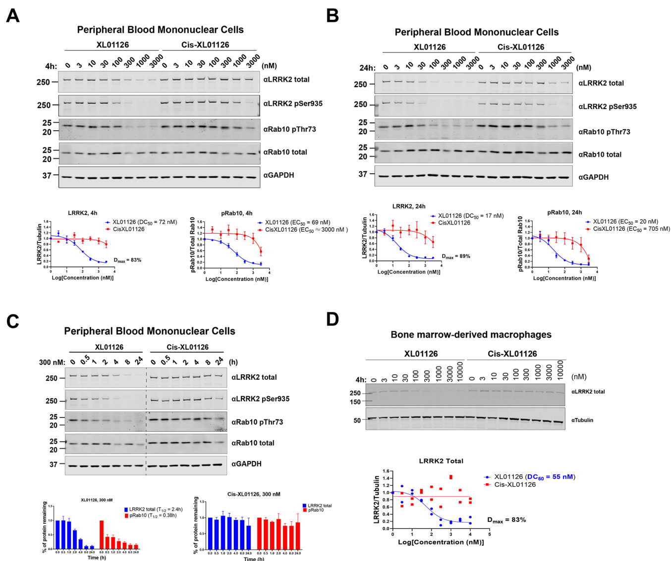
Figure 8. XL01126 degrades LRRK2 in human peripheral blood mononuclear cells (PBMCs) derived from healthy donors and mouse bone marrow-derived macrophages (BMDMs). Representative Western blotting of total LRRK2, LRRK2-pSer935, pRab10, Rab10 total, and GAPDH levels following treating the PBMCs with XL01126 and cis -XL01126 at the indicated concentrations for 4 h (A) and 24 h (B). The relative LRRK2 protein and pRab10 levels were obtained by quantifying the ratios of total LRRK2/GAPDH or Rab10-pThr73/total Rab10, respectively, and the ratios were normalized to the DMSO-treated samples. The relative LRRK2 protein and pRab10 levels were plotted against the compound concentration and fitted against "nonlinear regression, one site-fit log IC 50 " in GraphPad to obtain the DC 50 and EC 50 values. Data points are presented as mean ± standard error of the mean (SEM) from three biological independent replicates. (C) Representative Western blotting of total LRRK2, LRRK2-pSer935, pRab10, Rab10 total, and GAPDH levels following treating the PBMCs with 300 nM of XL01126 and cis -XL01126 for the indicated time periods. The relative LRRK2 protein and pRab10 levels were obtained by quantifying the ratios of total LRRK2/GAPDH or Rab10-pThr73/total Rab10, respectively, and the ratios were normalized to the DMSO-treated samples. The relative LRRK2 and pRab10 protein levels were plotted against the treatment time and were fitted against "nonlinear regression, one-phase decay" in GraphPad to obtain the half-life ( T_{1/2} ) values. Data points are presented as mean ± SEM from three biological independent replicates. (D) Representative Western blotting of LRRK2 total and tubulin levels after treating BMDMs with XL01126 and cis -XL01126 for 4 h. The relative LRRK2 levels were obtained by quantifying the ratios of total LRRK2/tubulin and normalized to the DMSO-treated samples. The relative LRRK2 levels were plotted against the compound concentration and fitted against "nonlinear regression, one site-fit log IC 50 " in GraphPad to obtain the DC 50 values.
