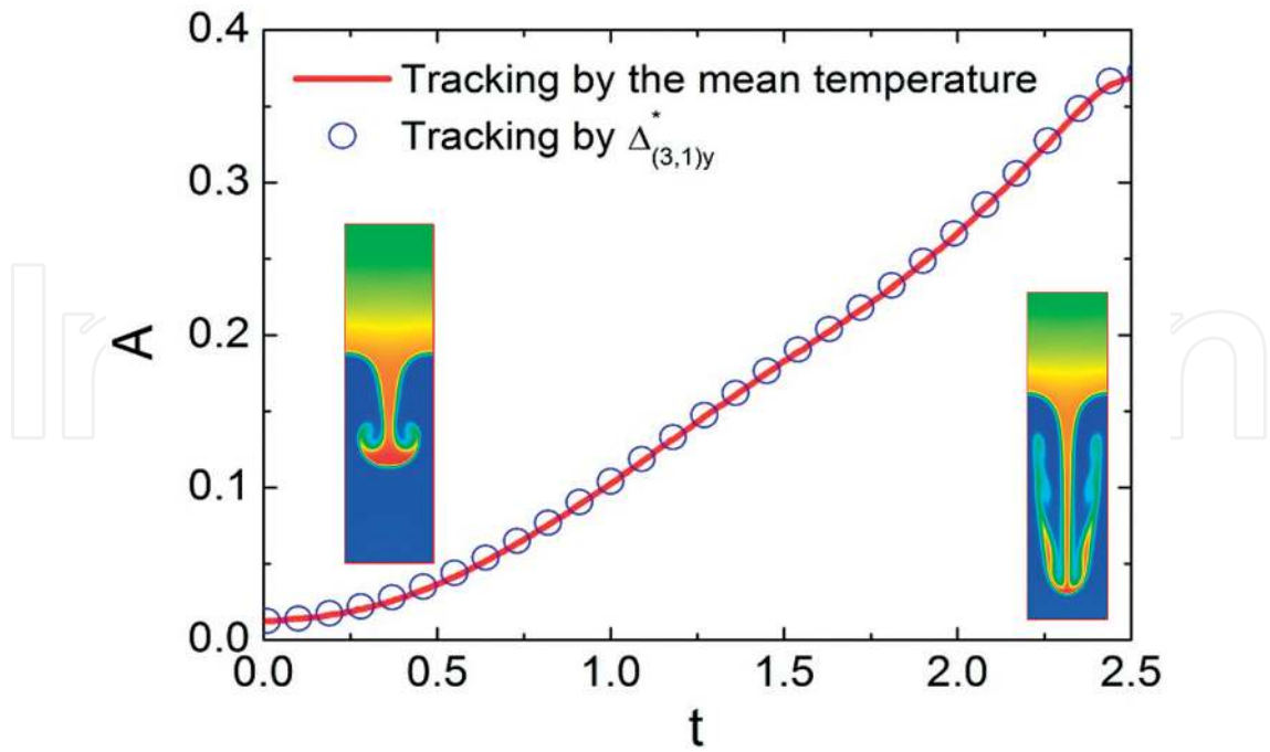
Figure 5. The perturbation amplitudes developing with time obtained by two different tracking approaches (see Ref. [23] for more details).
