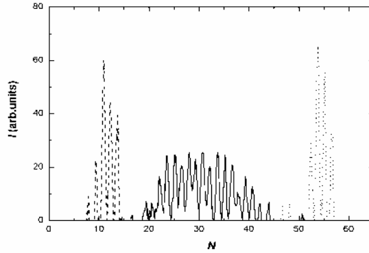
Fig. 5. Probing diffraction in the periodic waveguide array by varying the angle of incidence of a four-channel input beam, from K_z = 0 (solid line), to nearly diffraction-free propagation at K_z \approx \pm \pi/2\Lambda (dotted and dashed lines).
