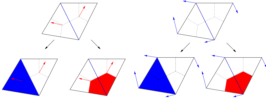
Figure 5.2: Top row: dual (left) and primal (right) vector fields X for which X^b is desired on the shared edge ; Bottom row: (left to right) dual-primal, dual-dual, primal-primal and primal-dual interpolations. See Def. 2.7.1 for more on interpolation. The bottom row corresponds to the configuration for the discrete flats b_{dpp} , b_{ddp} , b_{ppp} and b_{pdp} . A dual destination would yield 4 more flats for a total of 8 discrete flats.
