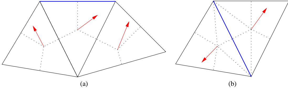
Figure 5.3: (a) For a boundary edge in 2D there is no ambiguity about the the dual vector field to use for defining a DPP-flat. The vector in the triangle containing the edge is used ; (b) On the shared edge the vector field is not well defined. In 2D the two values to choose from are in the triangles sharing the edge. See Fig. 5.4, Def. 5.5.2, and the explanation of that definition for a resolution of the ambiguity.
