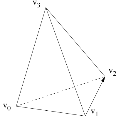
Figure 8.1: The configuration for computing the flow-out formula of Lie derivative of a 1-form. The vector field is nonzero only at v_1 and has the length and direction of the edge [v_1, v_2] . It is linearly interpolated to be 0 at vertex v_2 . This is the restriction, to an edge, of the barycentric interpolation of the vector field inside the tetrahedron. We wish to evaluate the Lie derivative of a 1-form on the edge [v_0, v_1] .
