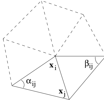
Figure 6.2: The variable names used in formula (6.4.1) for the Laplace-Beltrami of a triangle mesh, found by Meyer et al. [2002]. The complex does not have to be flat.
