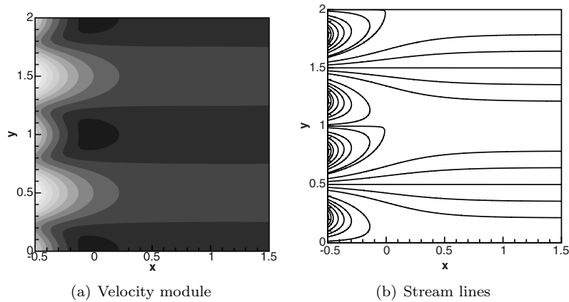
FIGURE 2. Plot of Kovaszny's solution for k = 1 and mesh 5.
