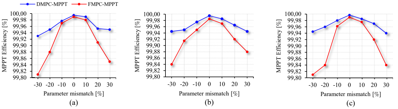
Fig. 14. Simulation results of FMPC-MPPT and DMPC-MPPT efficiencies under STC, and in case of model parameter mismatch using: (a) Boost converter “ L and C_3 ”, (b) Z-source inverter “ C_l and L_l ”, and (c) Flyback converter “ C and L_m ”.
