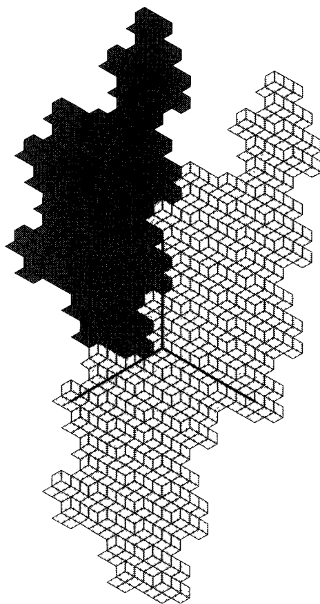
Figure 12. A neighbourhood of the origin obtained by iteration on four faces
