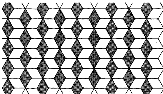
Figure 4. The lattice \Gamma
