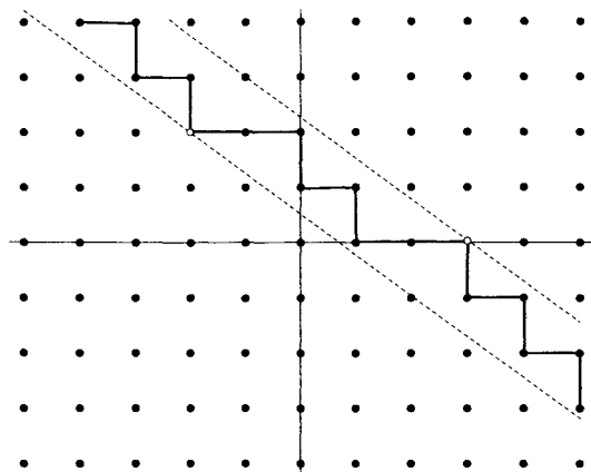
Figure 2. The discrete line: dual case
