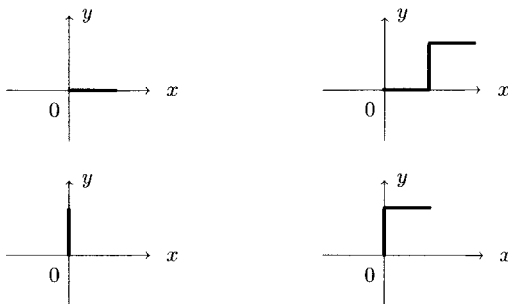
Figure 9. The one-dimensional extension of 0 \mapsto 010, 1 \mapsto 10
