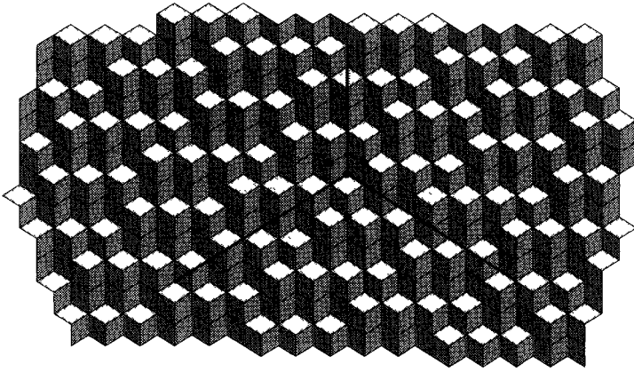
Figure 3. The stepped surface
