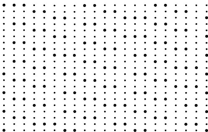
Figure 6. An induced orbit
