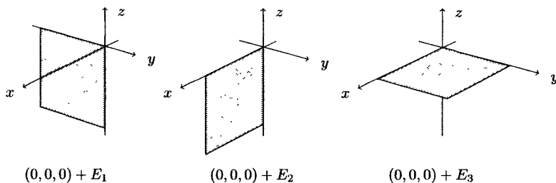
Figure 5. The three possible faces with distinguished vertex at the origin
