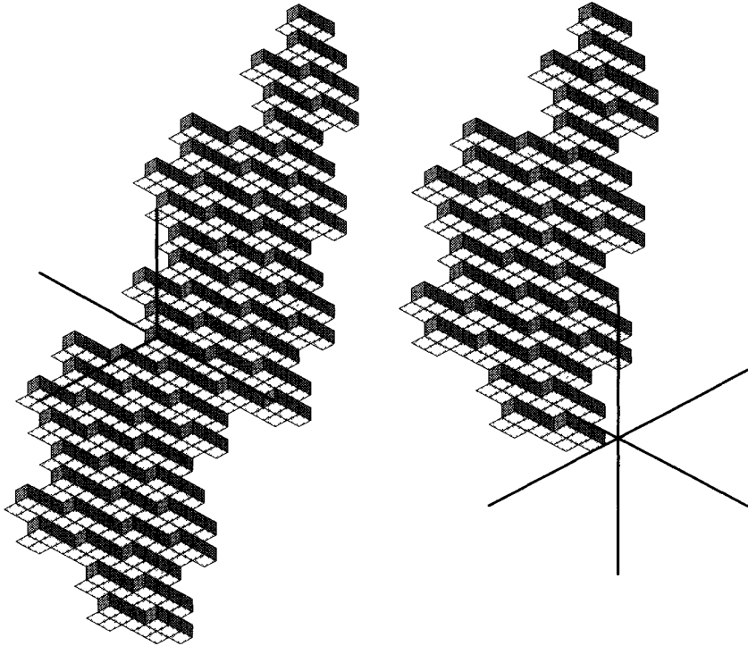
Figure 10 (left). Iteration starting from the faces at the origin
