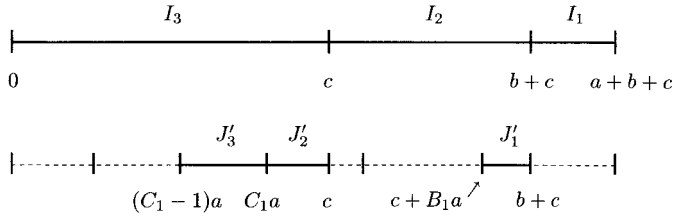
Figure 8. Induction on the interval J'
