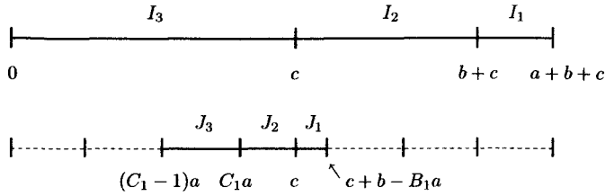
Figure 7. Induction on the interval J
