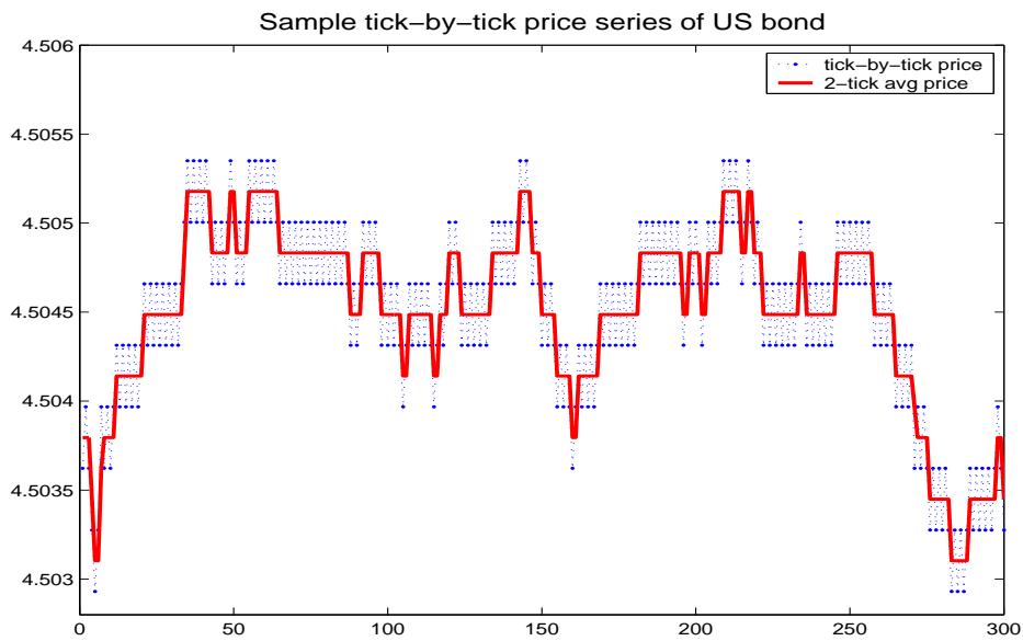
Figure 4: Sample path of the tick-by-tick price process (dotted line) with a its two ticks moving average (solid line) for the S&P 500 (top panel) and US Bond (bottom panel) future.
