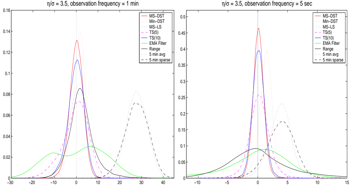
Figure 1: Comparison of the pdf of the estimation errors on the annualized percentage volatility (on average 20%) obtained with an average observation frequency of 1 minute (left panel) and 5 seconds (right panel) and a noise to signal ratio \frac{\eta}{\sigma} = 3.5 .
