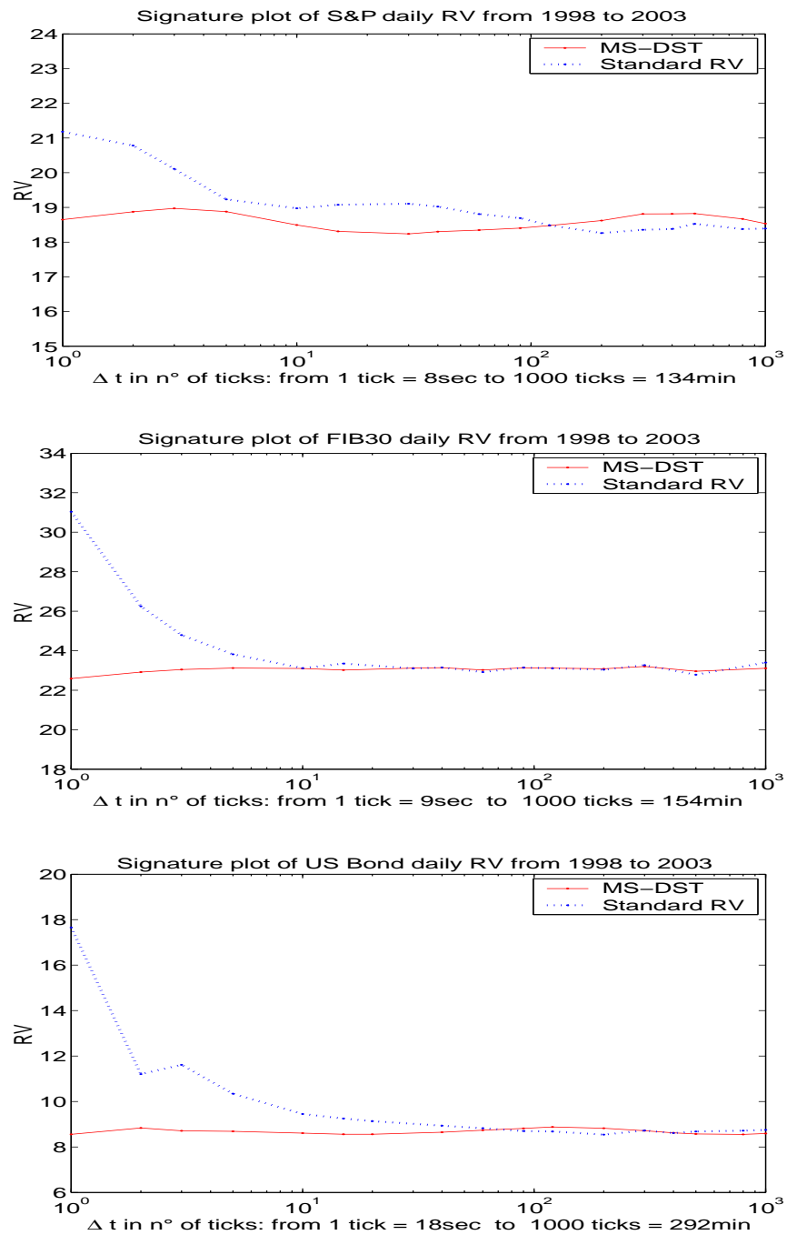
Figure 7: Signature Plot in semilog scale of the standard (dotted) and DST (solid) realized volatility for S&P 500, FIB 30 and US Bond from January 1998 to October 2003.
