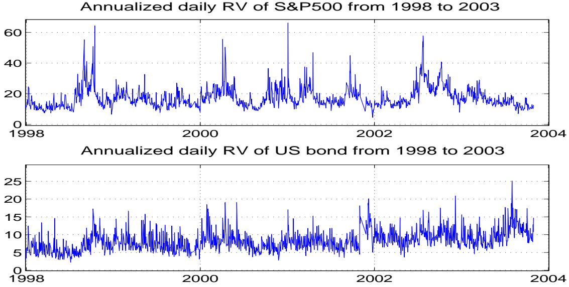
Figure 6: Time series of the annualize realized volatility computed with the MS-DST estimator on the two ticks returns for the S&P 500 (top panel) and US Bond (bottom panel) futures from 1998 to 2003.
