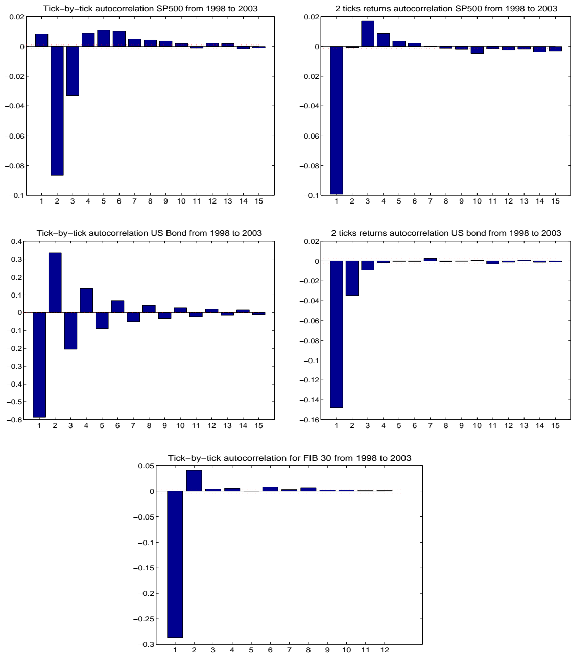
Figure 5: Sample autocorrelation of S&P (top) and US Bond (middle) for tick-by-tick returns (left) and 2-ticks returns (right) together with the tick-by-tick autocorrelation of FIB30 (bottom). All autocorrelation functions are computed over the six year sample, from 1998 to 2003.
