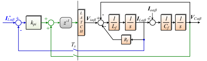
Fig. 15. Block diagram of the physical system with current loop only, latch interface and one sample delay.
