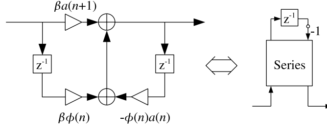
Figure 41. A signal flow diagram of a wave digital one-port implementation (left) and its abstraction (right). The one-port acts as an energy-preserving fractional delay even when a(n) varies in time. If a(n) is constant, the structure reduces to a first-order allpass filter. The filter coefficients are evaluated as in equation (109).
