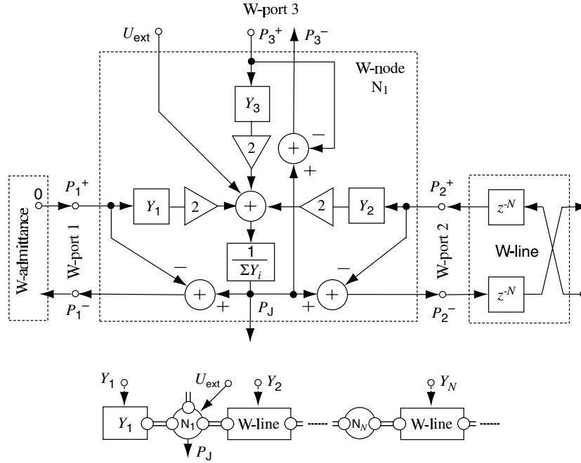
Figure 13. Top: a 3-port parallel scattering junction for acoustic pressure waves. Incoming pressures are P_i^+ , outgoing ones P_i^- and P_J is common junction pressure. Port 1 (left) is terminated by admittance Y_1 , port 2 (right) is connected to a delay-line having wave admittance Y_2 , and port 3 (top) is not connected. Bottom: block diagram with abstracted block notation and how the blocks can be connected to form a 1D digital waveguide.
