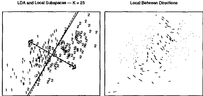
Figure 3: [Left Panel] Two dimensional gaussian data with two classes and correlation 0.65. The solid lines are the LDA decision boundary and its equivalent subspace for classification. The dashed lines were produced by the local procedure described in this section. [Right panel] Each line segment represents the local between information centered at that point.
