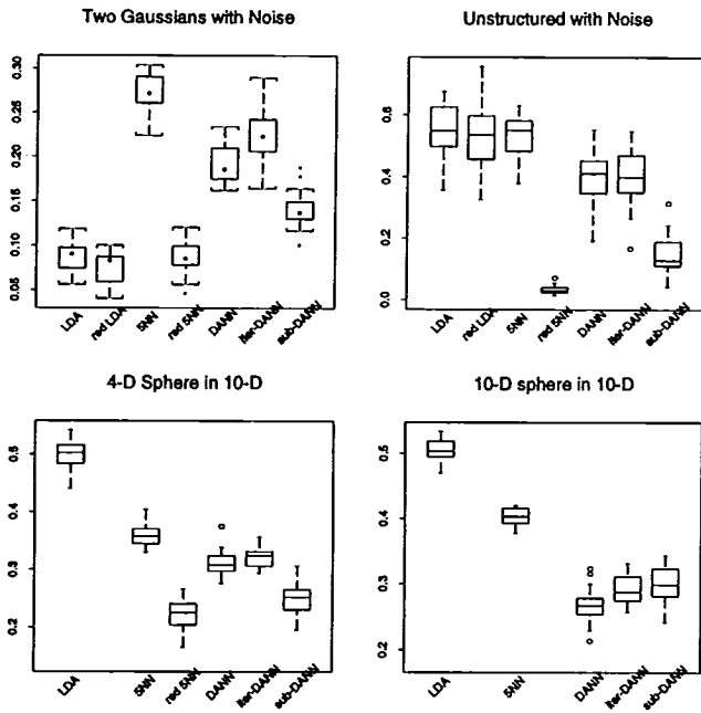
Figure 5: Boxplots of error rates over 20 simulations.
