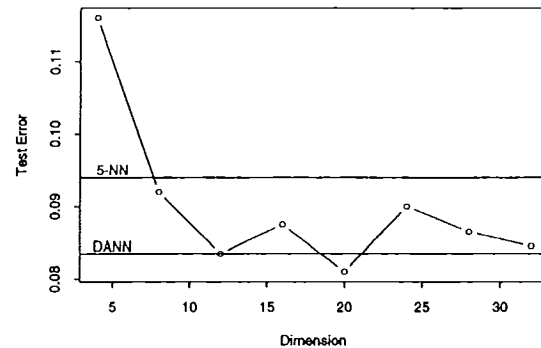
Figure 10: Misclassification results as a function of subspace size, for the satellite image data
