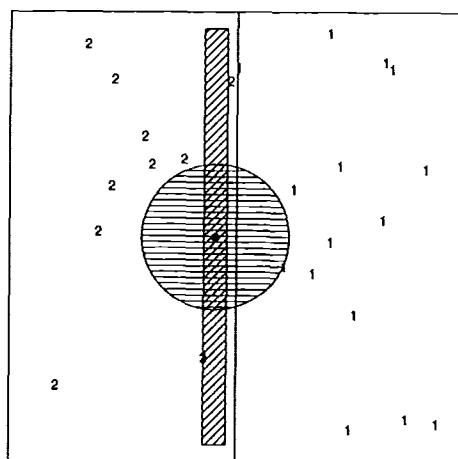
Figure 1: The vertical strip denotes the NN region using only the X coordinate to find the nearest neighbor for the target point (solid dot). The sphere shows the NN region using both coordinates, and we see in this case it has extended into the class 1 region (and found the wrong class in this instance).
