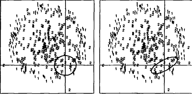
Figure 2: The left panel shows a spherical neighborhood containing 25 points. The right panel shows the ellipsoidal neighborhood found by the DANN procedure, also containing 25 points. The latter is elongated along the true decision boundary, and flattened orthogonal to it.
