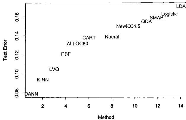
Figure 9: Misclassification results of a variety of classification procedures on the satellite image test data (taken from Michie et al. (1994)).
