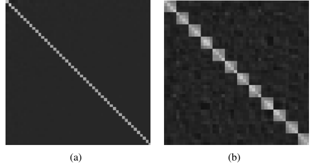
Fig. 1. Visualization of covariance matrices (black color represents zero values and the elements with higher values are illustrated brighter). (a) Covariance between features ( \tilde{X} \tilde{X}^{*T} ). (b) Covariance between samples ( \tilde{X}^{*T} \tilde{X} ).
