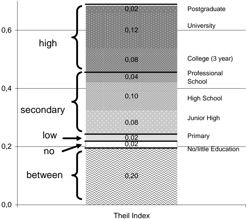
Figure 1: Theil Index by education groups
