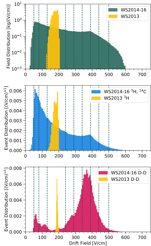
FIG. 1. The distribution of drift fields in the LUX datasets. (Top) The mass distribution of field within the LUX fiducial volume. In this analysis, we define the WS2013 fiducial volume as r < 20 cm and 38 < (t_{\text{drift}}/\mu\text{s}) < 305 , and the WS2014–16 fiducial volume as r < 20 cm and 40 < (t_{\text{drift}}/\mu\text{s}) < 300 . (Middle) For each electronic recoil, the field at the recoil site is calculated using the results of [32], and we plot a normalized histogram of the results. The ^3\text{H} and ^{14}\text{C} datasets are combined for WS2014–16 because they both fill the entire detector volume, and thus have identical distributions. Black dashed lines are used to indicate the field bins used in Section II. The WS2013 and WS2014–16 histograms are normalized separately in order to visualize the data effectively, so the relative heights of the blue and yellow histograms should not be considered an expression of the number of events in each dataset. (Bottom) The same as the middle panel, but for nuclear recoils.
