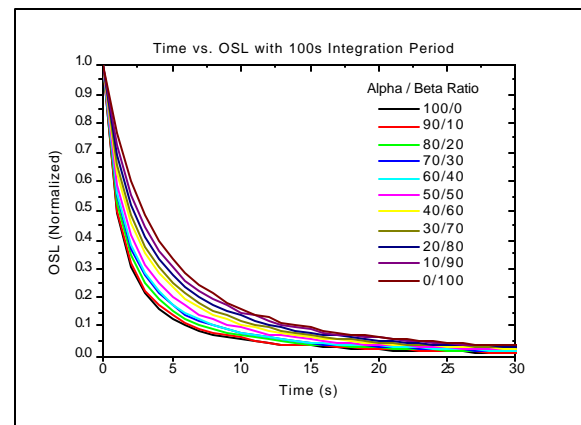
Figure 1: OSL luminescence decay curves of samples irradiated with mixed \alpha and \beta particles ranging from 100% \beta (bottom) to 100% \alpha (top), normalized to their initial intensity.
