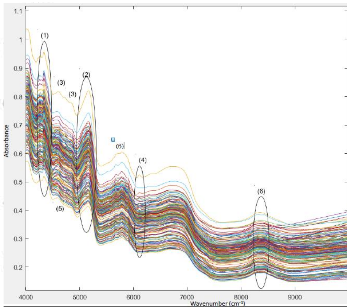
Fig.1 : NIR absorbance raw spectra obtained with the benchtop in the wavenumber region 10,000 – 4,000 \text{cm}^{-1} (A) and the dispersive absorbance raw spectra obtained with the handheld in the wavenumber region 6,000 – 4,000 \text{cm}^{-1} (B).
