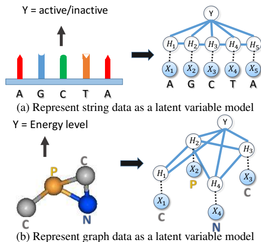
Figure 1. Building graphical model with hidden variables from structured string and general graph data. Y is the supervised information, which can be real number (for regression) or discrete integer (for classification).
