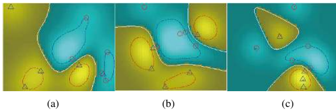
Fig. 5. RF models (i.e., the SVM hyperplane) are diverse with different semantic subspaces of feedback samples.
