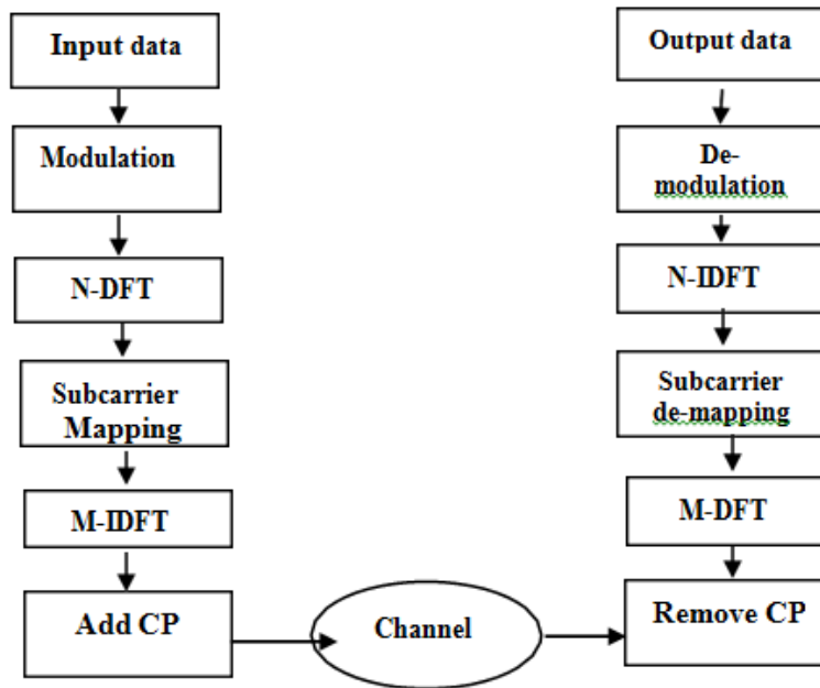
Figure 1: Simplified block diagram of the LTE SC wireless.
