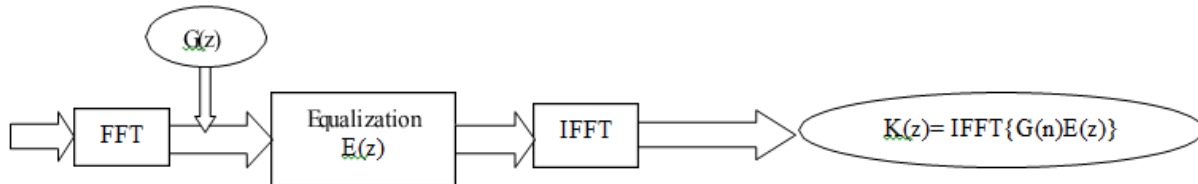
Figure 6: The process of channel equalization.
