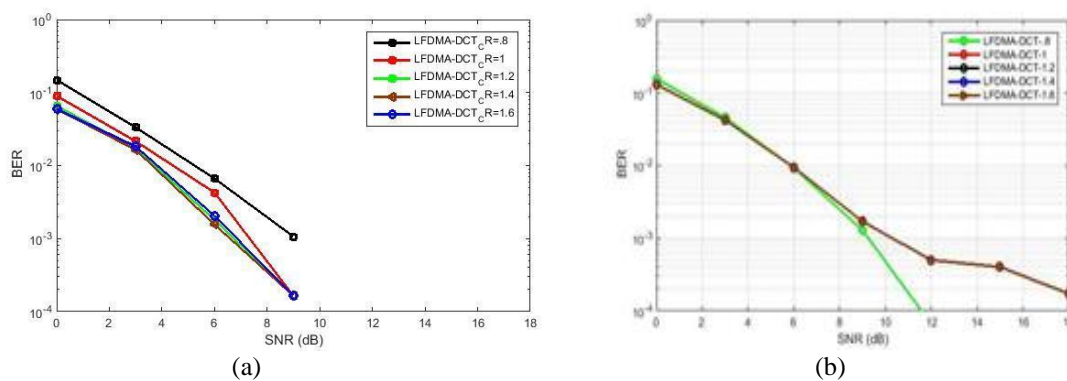
Figure 15: DCT results with SUI3 channel (a) Clipping and filtering (b) Clipping only.
