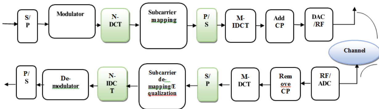
Figure 4: Structure of DCT-SC-FDMA system over a frequency-selective channel.
