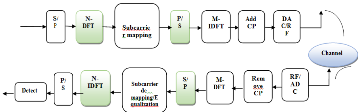
Figure 2: SC-FDMA transmit-receive system.
