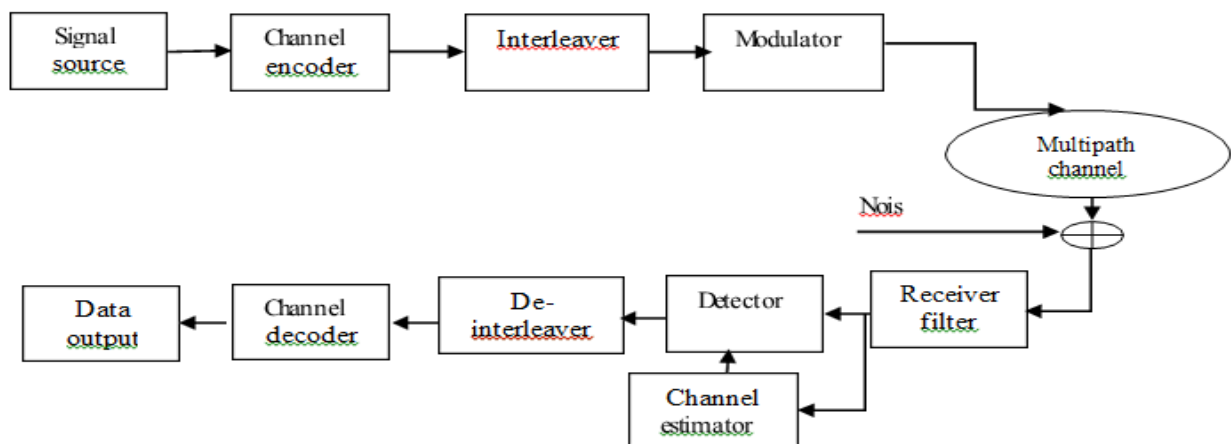
Figure 5: Block diagram for a system utilizing channel estimator and detection.
