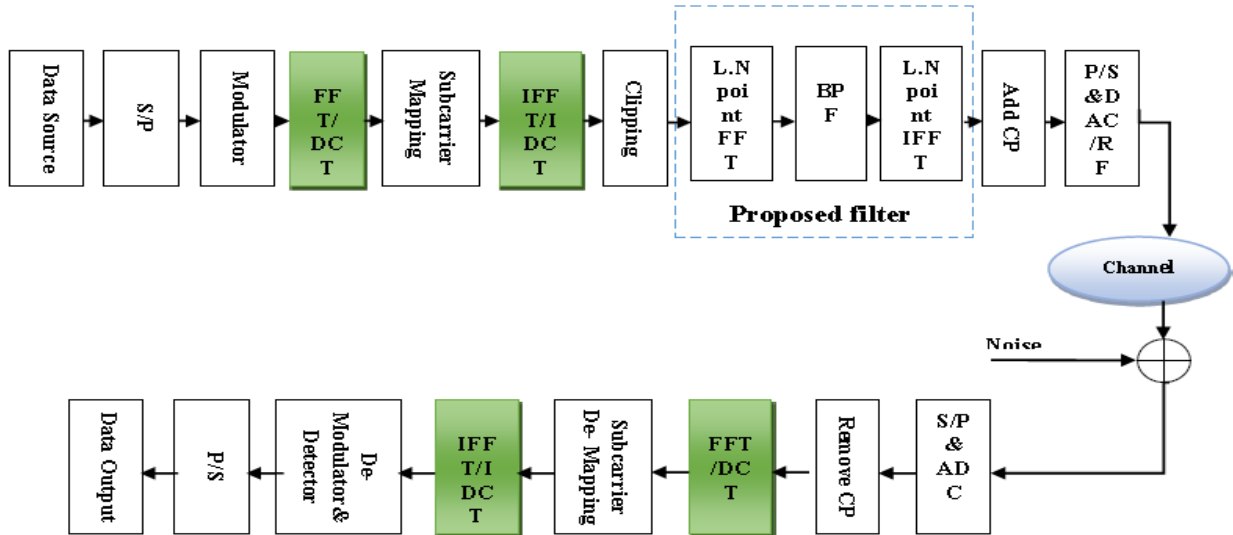
Figure 9: The proposed SC-FDMA with Clipping and filtering system.
