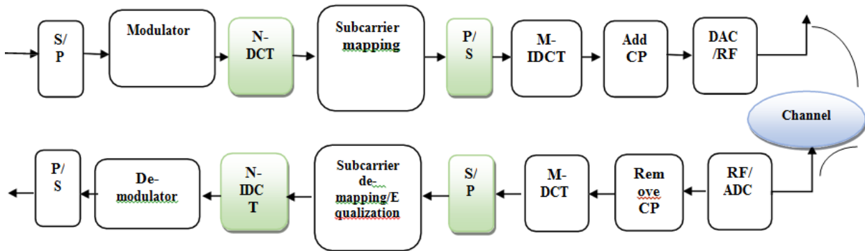
Figure 3: block diagram of the DFT-SC-FDMA system.
