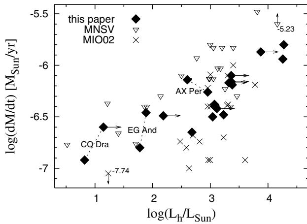
Fig. 24. Comparison of our mass-loss rates from Table 3 with those published by MNSV ( \nabla , recalculated to our d and v_\infty = 20 km s -1 ) and by Mikolajewska et al. (2002b) ( \times , obtained from radio observations and scaled with v_\infty = 20 km s -1 ). Horizontal arrows indicate a shift in the luminosity by a factor of 2 for values of T_h > T_h^{\text{min}} .
