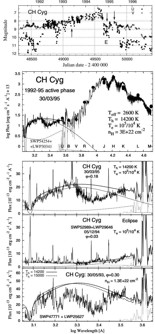
Fig. 9. Example of the SED for CH Cyg during its 1992–95 active phase. Spectra prior to, in and after the 1994 eclipse were selected. Corresponding dates are marked at the LC on the top panel.
