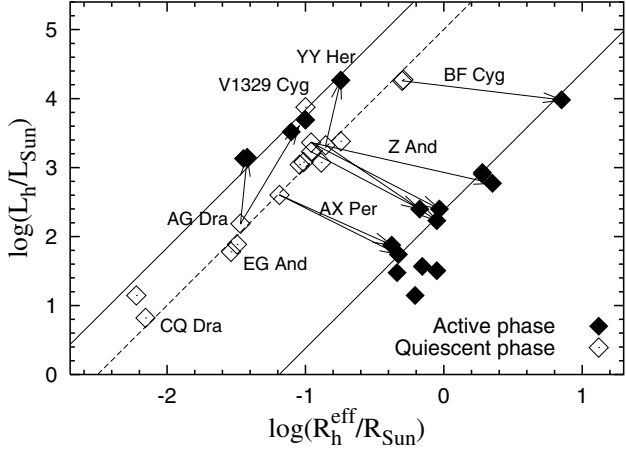
Fig. 26. The L - R relationship for the hot stellar component of radiation. It satisfies well radiation of stellar photospheres (Eq. (31)). During quiescence (open squares, dashed line) stellar components of investigated objects radiate at a characteristic temperature of \sim 103\,000 K, while during outbursts (filled squares, solid lines) this temperature decreases significantly to \sim 22\,000 K (1st-type of outbursts) or increases to \sim 165\,000 K (2nd-type of outbursts).
