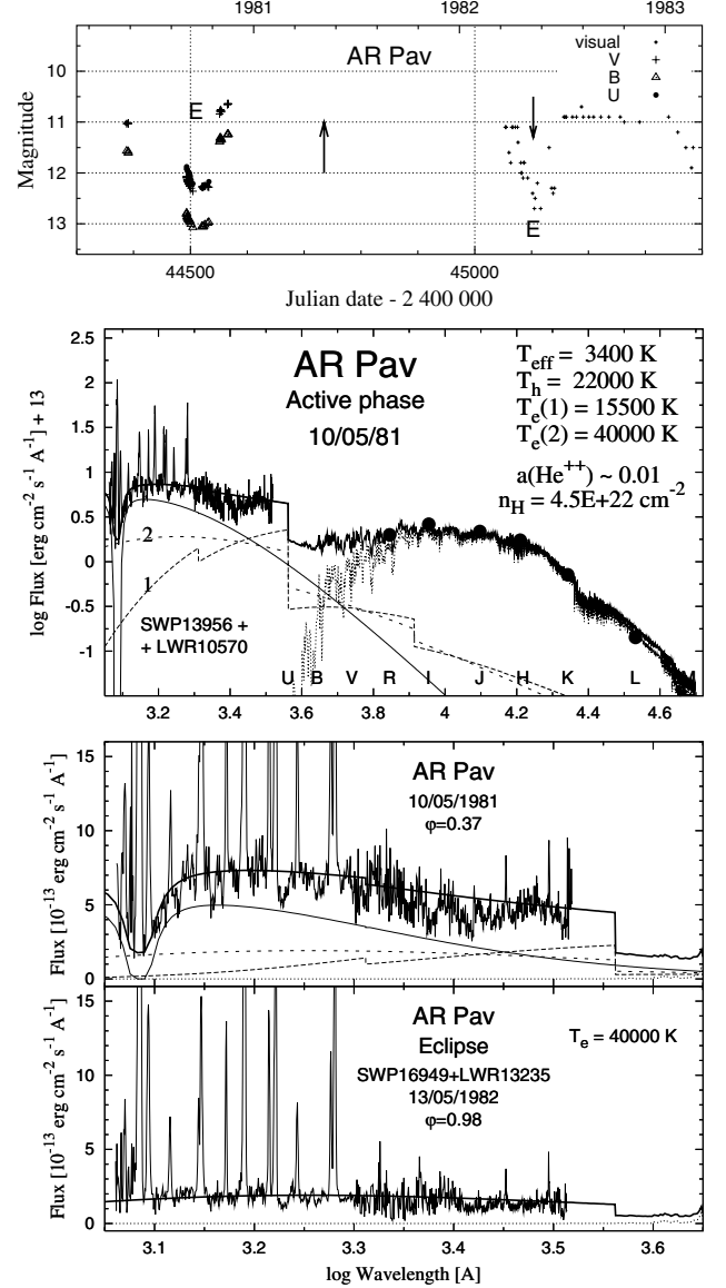
Fig. 19. The SED for AR Pav out and in the eclipse (positions of the spectra used are marked by arrows in the relevant part of the LC). Its out-of-eclipse profile in the ultraviolet resembles that observed in other eclipsing systems during active phases.
