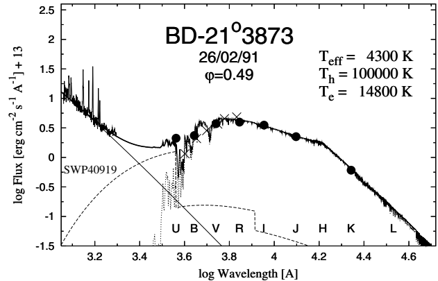
Fig. 22. Approximate SED for BD – 21°3873 given by its SWP spectrum in the ultraviolet and UBVRIJK fluxes from photometric measurements (●). The value of U(\varphi = 0.31) from Munari et al. (1992) was extrapolated to U(\varphi = 0.5) according to the profile of the u -LC. Crosses (×) represents flux-points from the spectrum taken on 24/02/88 ( \varphi = 0.61 ) by Niehues et al. (1992).
