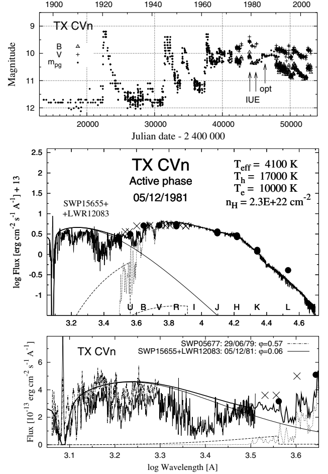
Fig. 6. The observed and modeled SED of TX CVn. The ultraviolet continuum is drastically affected by the iron curtain absorptions and the far-UV part is moderately attenuated by the Rayleigh scattering – typical features of active phases of symbiotic stars. Flux-points of the optical spectroscopy ( \times ) are from Kenyon & Garcia (1989). Dates of spectroscopic observations are marked by arrows at the top panel.
