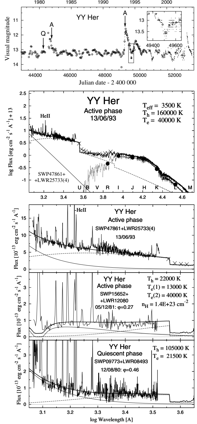
Fig. 16. The SED of YY Her during quiescence and two different phases of activity. Visual LC is composed from the data of Munari et al. (1997a) (○) and those available from the CDS database (●). The eclipse effect observed in 1994.43 is shown in detail. Crosses (×) in the SED represent continuum flux-points from the optical spectrum taken on 10/06/93 (Munari et al. 1997a).
