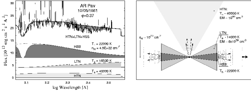
Fig. 27. Schematic representation of a basic structure of hot objects during outbursts of the 1st-type. The left panel shows example of individual components of radiation we isolated from the AR Pav spectrum observed on 10/05/81. Note that the HSS radiation is Rayleigh attenuated at the far-UV region and veiled by a forest of blended Fe II absorptions. The right panel shows a sketch of the corresponding emitting regions as seen on a cut perpendicular to the orbital plane containing the accretor. During outbursts the disk’s outer rim has to be flared to occult permanently the central source of the hot ionizing radiation. The model is described in Sect. 5.3.5.
