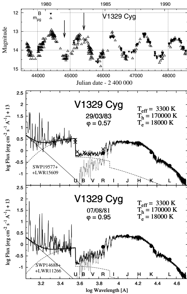
Fig. 11. The SED in the continuum of V1329 Cyg at maximum and minimum of the wave-like variation in the LC. Crosses (×) at the SED from the maximum represent continuum fluxes taken from the optical spectra presented in Figs. 192 and 193 of Munari & Zwitter (2002). Dates of the IUE observations are marked in the LC.
