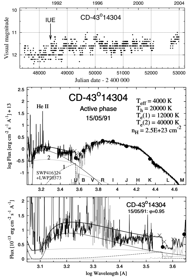
Fig. 5. The SED for CD 43° 14304. It is very similar to that from active phases of other well known systems. Crosses (×) represent fluxes in the continuum of the optical spectroscopy carried out in July 1991 (Gutiérrez-Moreno et al. 1999). At the time of IUE observations the system just entered an active phase ( top panel ).
