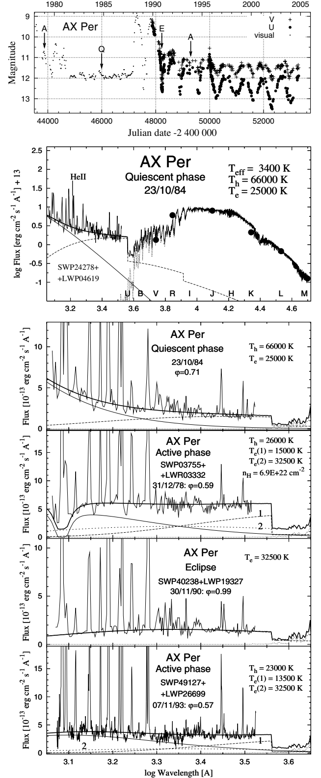
Fig. 21. The SED for AX Per during the activity, quiescence and eclipse. Positions of the spectra used are marked by arrows in the LC. Small dots represent means of the CDS visual data in the 30-day bins.
