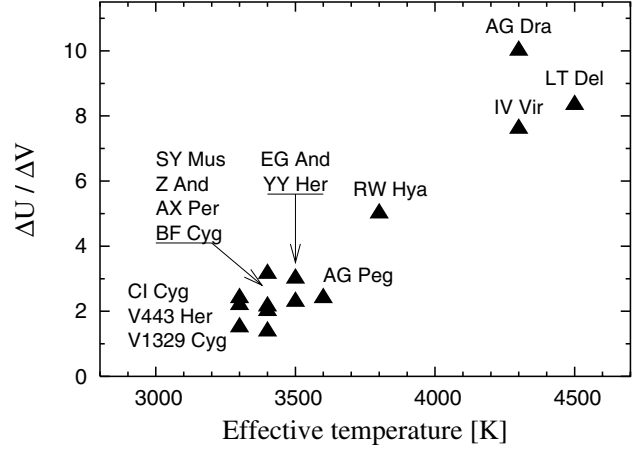
Fig. 25. Ratio of amplitudes in U and V of the orbitally-related variation in quiescent LCs as a function of the effective temperature of the giant. The ratio of fluxes from the giant and the nebula depends largely on the giant's effective temperature, which determines the overall relationship. Systems with a higher nebular emission have lower ratio of \Delta U/\Delta V for the given T_{\text{eff}} .
