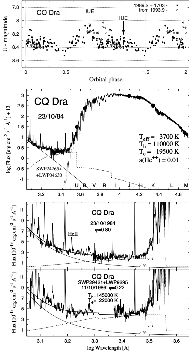
Fig. 14. The SED of CQ Dra from two shifts of the IUE satellite. A strong and variable nebular emission dominates the ultraviolet while in the optical/IR we can detect radiation from only the red giant. Variation in the U band reflects probably that in the nebular radiation. Optical photometry is from Hric et al. (1994).
