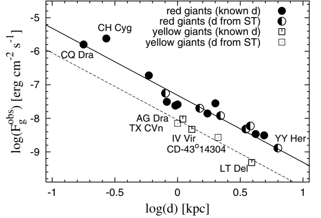
Fig. 23. The relationship between the observed bolometric flux of giants, F_g^{\text{obs}} and the distance d . Giants with independently known radii or distances are distinguished (see the text). Data are from Tables 1 and 2. Solid and dashed line correspond to their fit given by relations (27) and (28). CH Cyg was omitted in the fitting (see the text).
