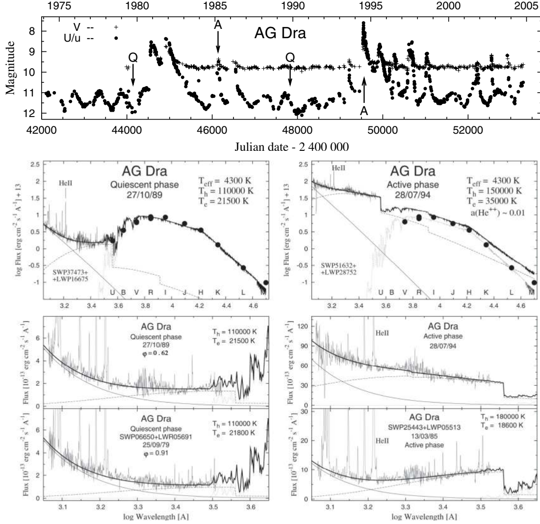
Fig. 13. The SED of AG Dra during quiescence ( left panels ) and active phases ( right ). Note the variation of the nebular emission and, in contrast, the stability of the hot stellar component with the orbital phase during quiescence. The SED during the active phases is characterized by a significant increase of the nebular emission, which constrains very high temperature of the ionizing source. Dates of the IUE observations are marked in the U/V LCs ( top ).
