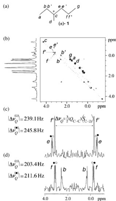
Figure 10: The distinction of a chiral alkane in PBLG/ \text{CDCl}_3 102 . The racemic mixture of compound (A) altogether shows 12 doublets in the Q-COSY spectrum for the ten hydrogens (B). Traces through deuterons e (C) and f (D) clearly indicate the distinction of the two enantiomeric species.
