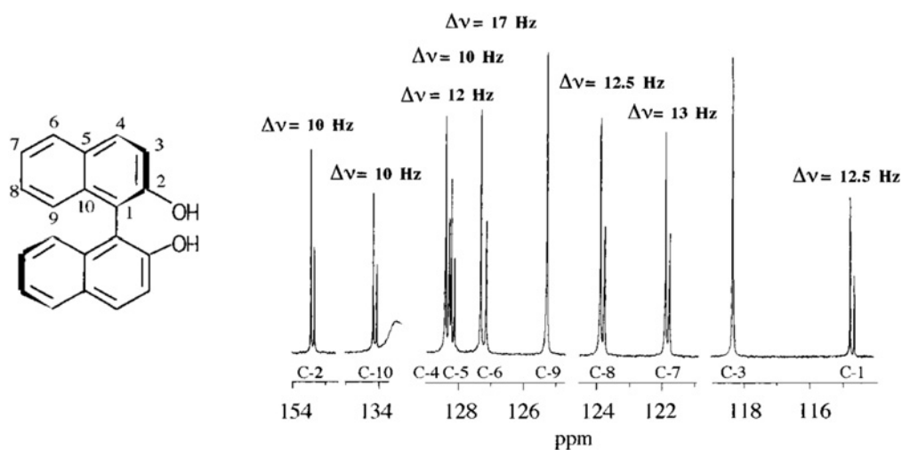
Figure 6: Distinction of the enantiomeric forms of 1,1'-bi-2-naphthol (see scheme to the left) in PBLG/DMF- d 7 using a 1 H-decoupled 13 C-1D-spectrum and differences in chemical shifts ( \Delta\nu indicated at each pair of signals). The weight in ee was 31% and integration determined 29.5% ee 57 .
