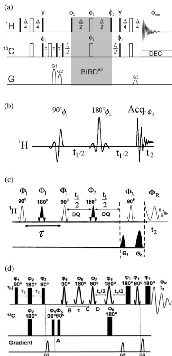
Figure 7: Experiments for enantiomeric distinction based on residual dipolar couplings. (A) 2D-version of a JE-BIRD d,x -HSQC experiment 40,41,69 ; (B) the selective 2D-SERF experiment using shaped excitation and refocussing pulses 71 ; (C) the selective DQ-SERF experiment 77 which can also be applied with higher order multiple quantum filtering 78 ; (D) the corresponding CH-DQ-SERF experiment for filtering of heteronuclear double quantum 81 . For phase cycling and further experimental details we refer the reader to the references specified.
