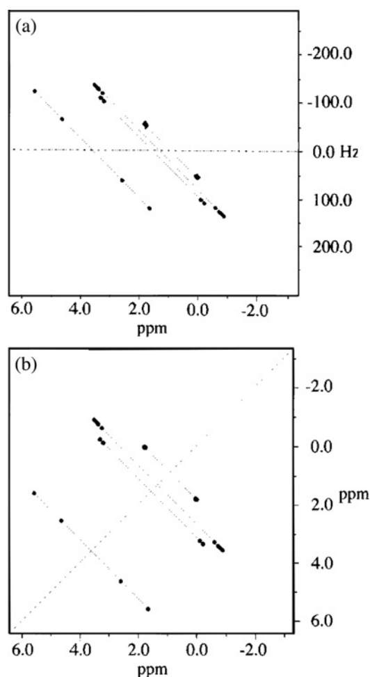
Figure 5: Application of the Q-COSY (A) and Q-resolved (B) experiments from Figure 4 to 1-pentanol- d_{12} in PBLG/ CDCl_3 . 55
