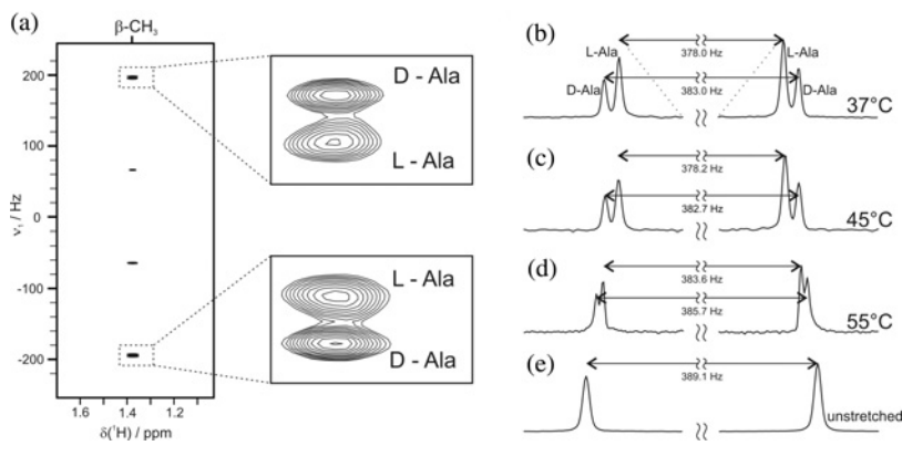
Figure 10: The distinction of a chiral alkane in PBLG/ \text{CDCl}_3 102 . The racemic mixture of compound (A) altogether shows 12 doublets in the Q-COSY spectrum for the ten hydrogens (B). Traces through deuterons e (C) and f (D) clearly indicate the distinction of the two enantiomeric species.
