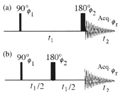
Figure 4: The Q-COSY (A) and Q-resolved (B) 2D pulse sequences for most efficient enantiomeric discrimination using deuterium quadrupolar couplings. For phase cycling and further experimental details the reader is referred to 55 .
