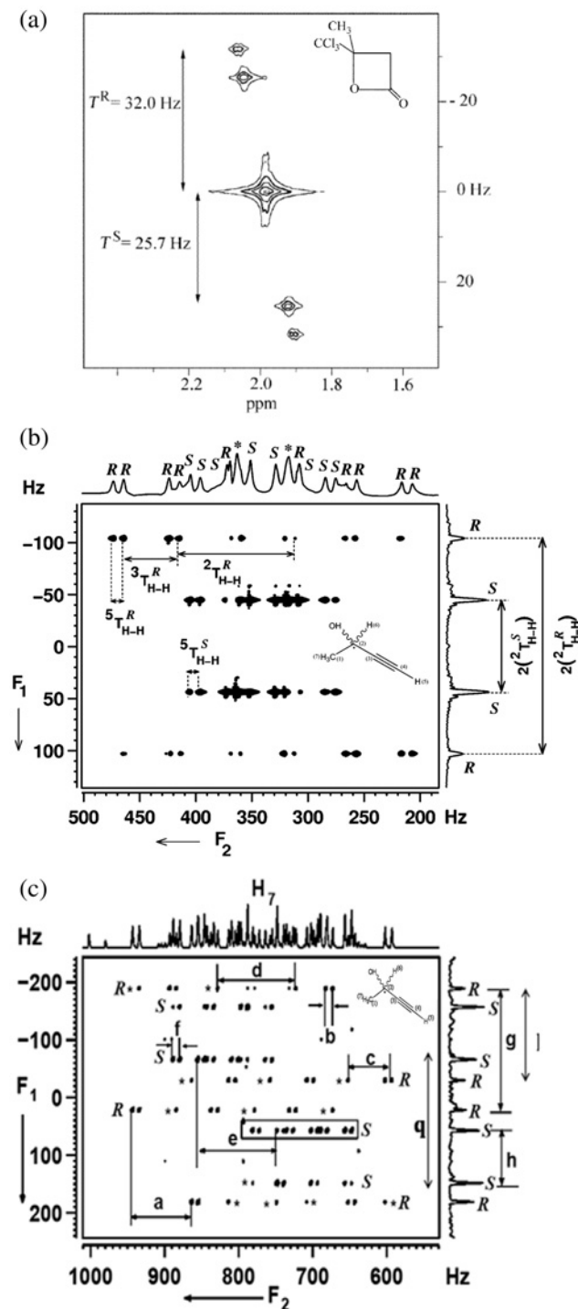
Figure 8: Experimental examples for the 2D-SERF 71 (Figure 7B), the DQ-SERF 77 (Figure 7C), and the CH-DQ-SERF 81 (Figure 7D) experiments. Corresponding example molecules are given as small insets. For further information regarding the indicated coupling constants the reader is referred to the cited references.
