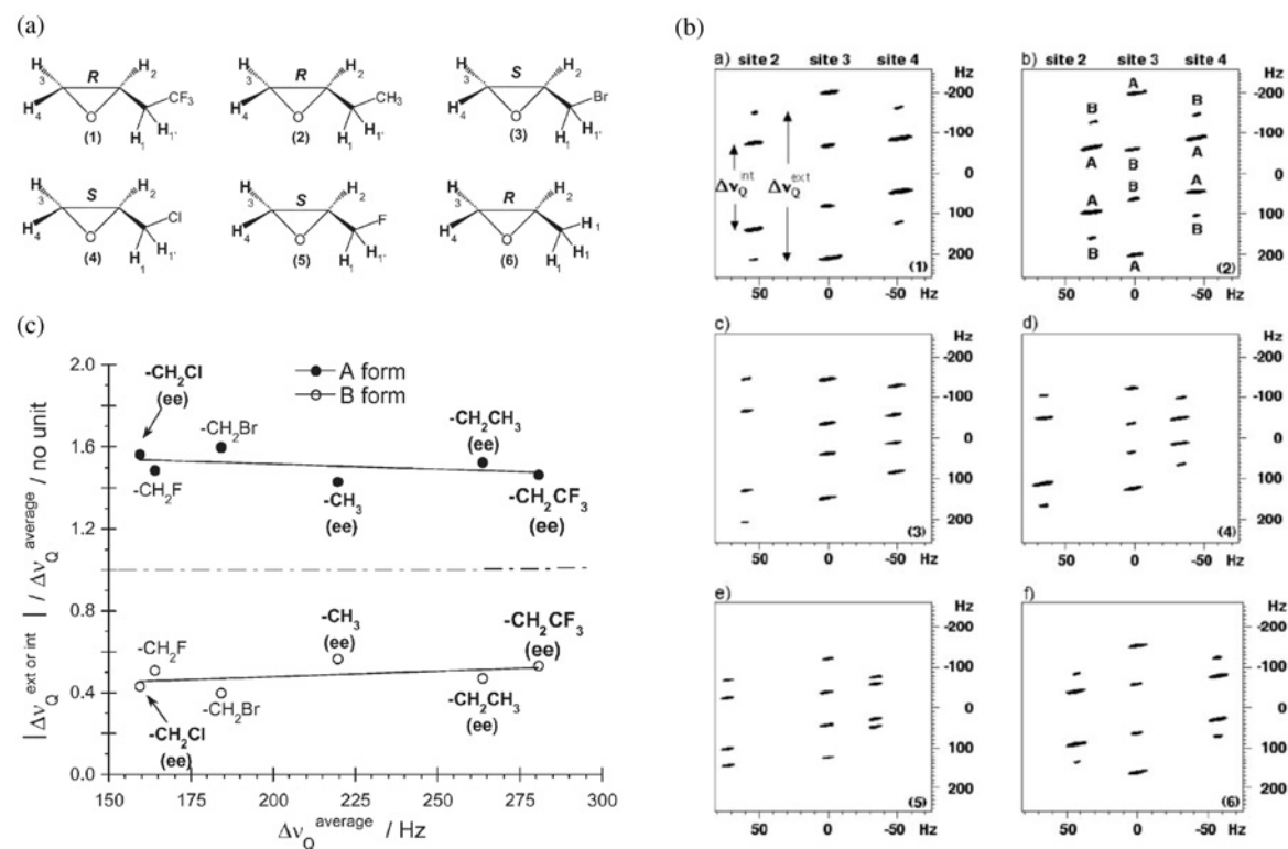
Figure 11: Determination of absolute chirality of an epoxide by comparison of deuterium quadrupolar couplings with similar compounds of known chirality 104 . (A) A-forms of the 6 enantiomeric pairs used in the study, from which the absolute chirality shall be determined for compound (1). Form B corresponds to the case where the substituent is behind the epoxide cycle. (B) The six corresponding natural abundance deuterium Q-COSY experiments with racemic mixtures of compounds (3) and (5) and A-form-enriched mixtures for (2),(4),(6). (C) The comparison of the normalized ratios of quadrupolar splittings clearly distinguishes A- from B-form and allows the secure determination of absolute chirality.
