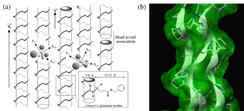
Figure 1: Helical secondary structures of PBLG and gelatin. (A) Ordered \alpha -helices of the liquid crystalline phase of PBLG 21 ; (B) the triple helix of gelatin.
