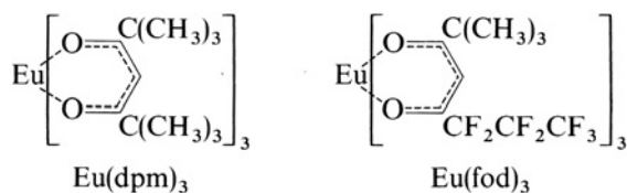
Figure 2: The two most widely used lanthanide shift reagents.
