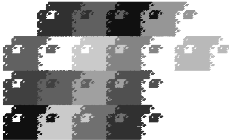
Fig. 2. A disconnected tile with six neighbors.
