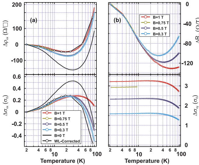
FIG. 2 (color). Magnetic field and temperature dependence of the full resistivity tensor for sample S1. (a), top. Temperature dependence of \tilde{\rho}_{xx} where WL effects have been suppressed analytically (labeled as “WL corrected”) and experimentally. WL was substantially suppressed at B = 300 mT and for B = 1 T, \Delta\tilde{\rho}_{\text{WL-Fit}} \approx \Delta\tilde{\rho}_{\text{WL-Exp}} . (a), bottom. The corresponding conductivity, \sigma_{xx} = \tilde{\rho}_{xx}/(\tilde{\rho}_{xx}^2 + \rho_{xy}^2) , in units of \sigma_0 = 2e^2/h \approx (12906.4 \text{ } \Omega)^{-1} . (b), top. Temperature dependence of the Hall coefficient R_H and the transversal conductivity (bottom) \sigma_{xy} = \rho_{xy}/(\tilde{\rho}_{xx}^2 + \rho_{xy}^2) in units of \sigma_0 .
