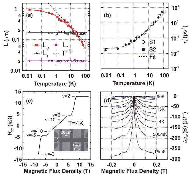
FIG. 1 (color). Magnetotransport measurements in monolayer SiC/G. (a) Temperature dependence of the characteristic scattering lengths and (b) decoherence rate ( \tau_\phi^{-1} ) for samples S1 (open markers) and S2 (solid markers). Dotted line is the fit to \tau_\phi^{-1} = \tau_s^{-1} + AT , with \tau_s^{-1} = 0.02 \text{ ps}^{-1} and A = 0.036 \text{ ps}^{-1} \text{ K}^{-1} . (c) Half-integer QHE proving the monolayer nature of SiC/G. Inset: Micrograph of one of the devices. (d) Weak localization peak at different temperatures.
