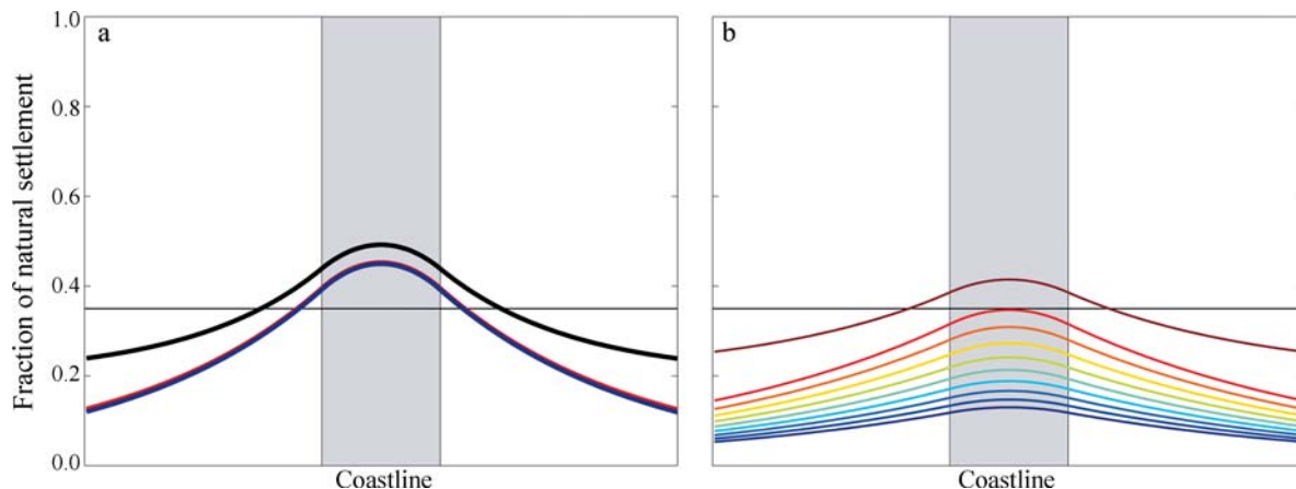
FIG. 3. Iterations of DPR_n for dispersal distances of (a) 1.1 and (b) 1.6 times the width of the reserve (shown in gray). Only every fifth DPR_n iteration is shown in (a) and (b). In total, 10 curves are shown in each panel. The first curve in both panels is DPR_{sat} and is identical in appearance to the corresponding curve in Fig. 2. In (a), DPR_n reaches the equilibrium settlement level in 5–10 iterations (the second and third curves), and therefore, some of the 10 curves cannot be seen as they are covered by higher iterations.
