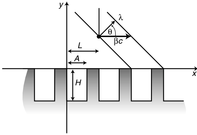
FIG. 1. Smith-Purcell radiation.
