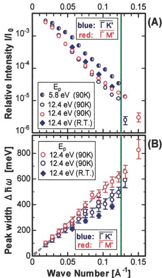
FIG. 3 (color). (A) Relative loss intensity plotted as a function of wave number q_{||} . (B) Plasmon linewidth plotted as a function of q_{||} . The Landau edge, q_c , is indicated by the green lines.
