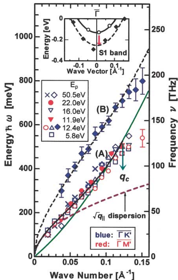
FIG. 2 (color). Plasmon dispersions measured at 90 K from (A) the “pristine” \sqrt{3} \times \sqrt{3} surface (1 ML) and (B) the \sqrt{3} \times \sqrt{3} surface decorated with 0.15 ML of additional Ag (1.15 ML in total). Blue and red plots represent the data obtained by scanning q_{||} along the \Gamma K' and \Gamma M' directions, respectively. The bold solid and dashed curves are the fits by full RPA dispersion. The green curve is the upper edge of the single-particle excitation continuum and the green arrow indicates the Landau edge, q_c , calculated for the pristine surface. The inset is a 2D band dispersion diagram showing the “sinkage” of the S1 band (the solid curve corresponds to the pristine surface, and the dashed curve corresponds to the adatom-decorated surface) [11].
