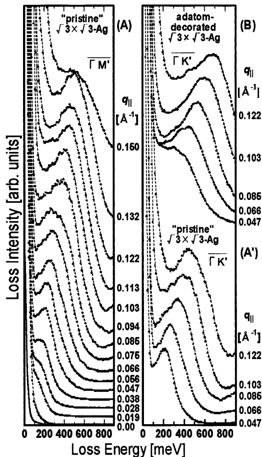
FIG. 1. Angle-resolved EELS spectra taken with electron primary energy E_p = 12.4 eV. (A) An example of q_{||} scanning along the \Gamma M' direction is shown. (A') and (B): The blueshift in energy dispersion due to the additional adatom decoration is demonstrated. Each spectrum was magnified to compensate for the intensity drop as a function of q_{||} .
