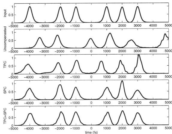
Fig. 3. Input and output pulses, with and without compensation schemes, when multiple 200-fs solitons propagate for a total distance of 1 km.
