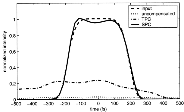
Fig. 2. Input and output pulses, with and without compensation schemes, when a 1.7-W 200-fs super-Gaussian pulse propagates for a total distance of 2 km.
