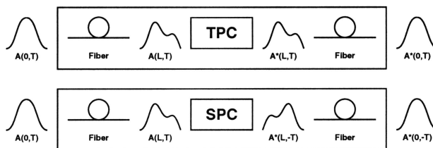
Fig. 1. Schematics of TPC and SPC.
