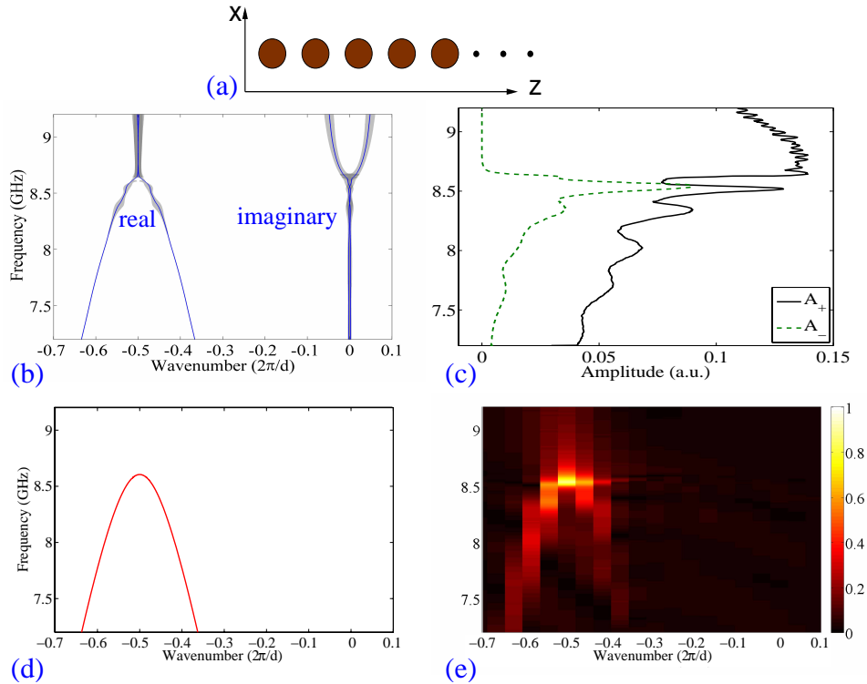
Fig. 1. (a) Sketch of the periodic waveguide made of dielectric pillars. (b) Dispersion retrieved from experimental measurements, shown are both the real and imaginary parts as indicated by labels. Grey shading marks the confidence interval. (c) Retrieved amplitudes of experimentally excited forward ( A_+ ) and backward ( A_- ) waves. (d) Numerically calculated dispersion. (e) Normalized SFT of experimentally measured electric field profile at rod centers along the waveguide.
