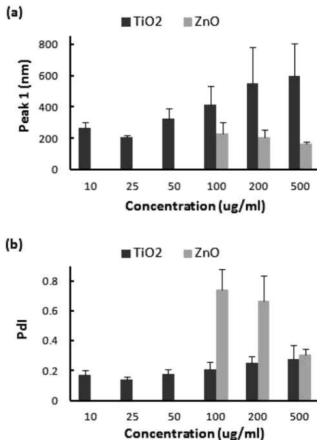
Fig. 1. Size characterization of TiO 2 and ZnO nanoparticle suspensions at concentration of 0.5 mg/ml dispersed by a probe-type sonicator at 20 W, 80% pulse mode, for 30 min, being measured by DLS at concentrations of 10, 25, 50, 100, 200, and 500 \mu\text{g/ml} : (a) peak 1 and (b) Pdl. Data are mean \pm SD.
