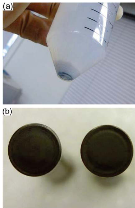
Fig. 6. (a) Black sediment at the bottom of a sample sonicated by a probe-type sonicator at 20 W, 80% pulse mode, for 30 min after 2 hours on standing and (b) the tip surface of unused probe (left) and abraded probe (right).
