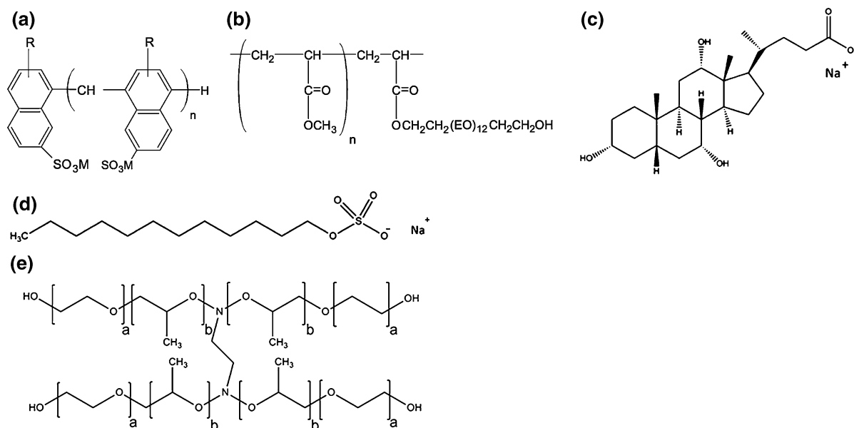
Fig. 2 Chemical structures of surfactants: a naphthalene-based superplasticizer and b polycarboxylate-based superplasticizer [35]; c SC, d SDS, and e Tetricon
