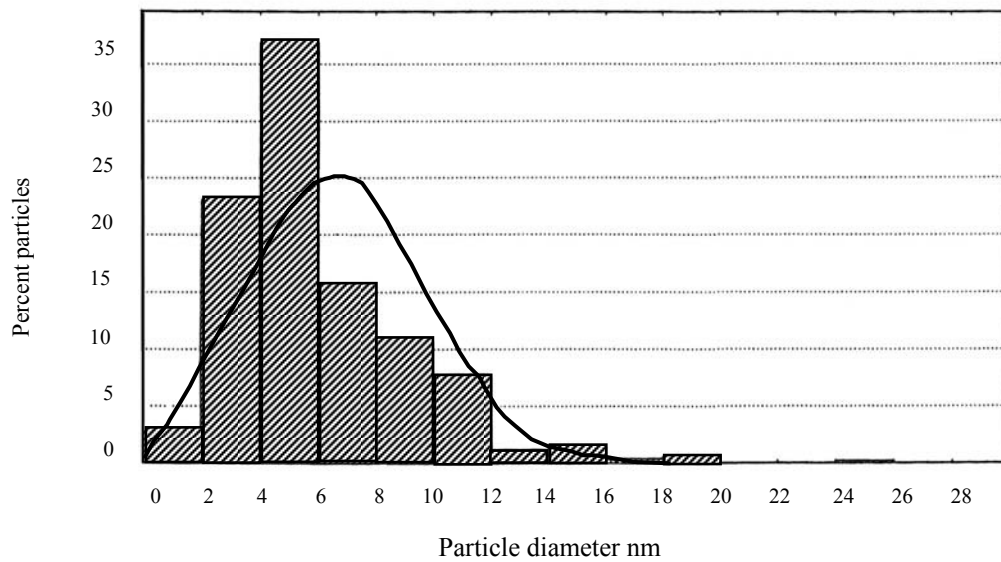
Fig 4 Experimentally determined size distribution for small particles for Steel V-N, equalisation temperature 1050^{\circ}\text{C} and end cool temperature 750^{\circ} , with an average particle diameter of 6.5nm.
