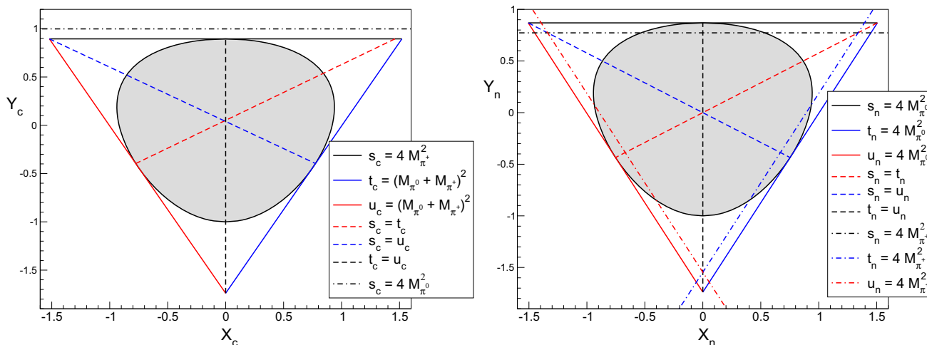
Fig. 6 The left panel shows the Dalitz plot geometry for the decay \eta \rightarrow \pi^+\pi^-\pi^0 in the plane of the two independent variables X_c, Y_c . The shaded area indicates the physical region, the full lines that are tangent to this region represent singularities generated by the final state interaction. In addition to the branch cut at s_c = 4M_{\pi^+}^2 (full), the s -channel contains a further such singularity outside the physical region, at s_c = 4M_{\pi^0}^2 (dash-dotted). The right panel shows the kinematics of
