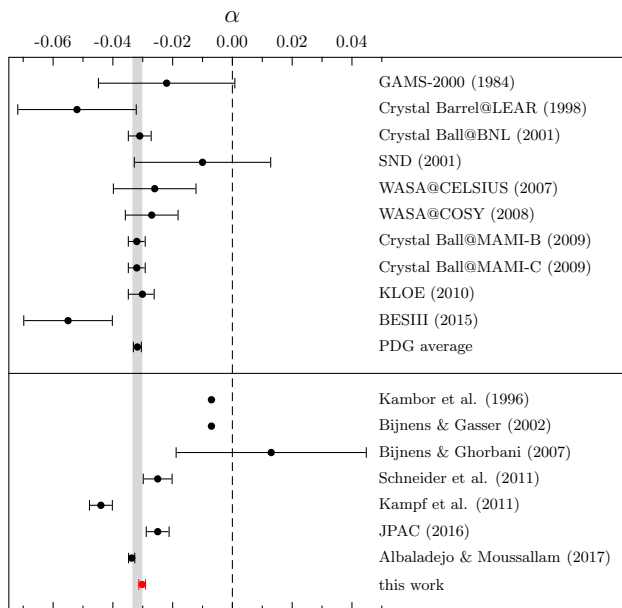
Fig. 15 Comparison of experimental and theoretical results for the slope \alpha of \eta \rightarrow 3\pi^0
