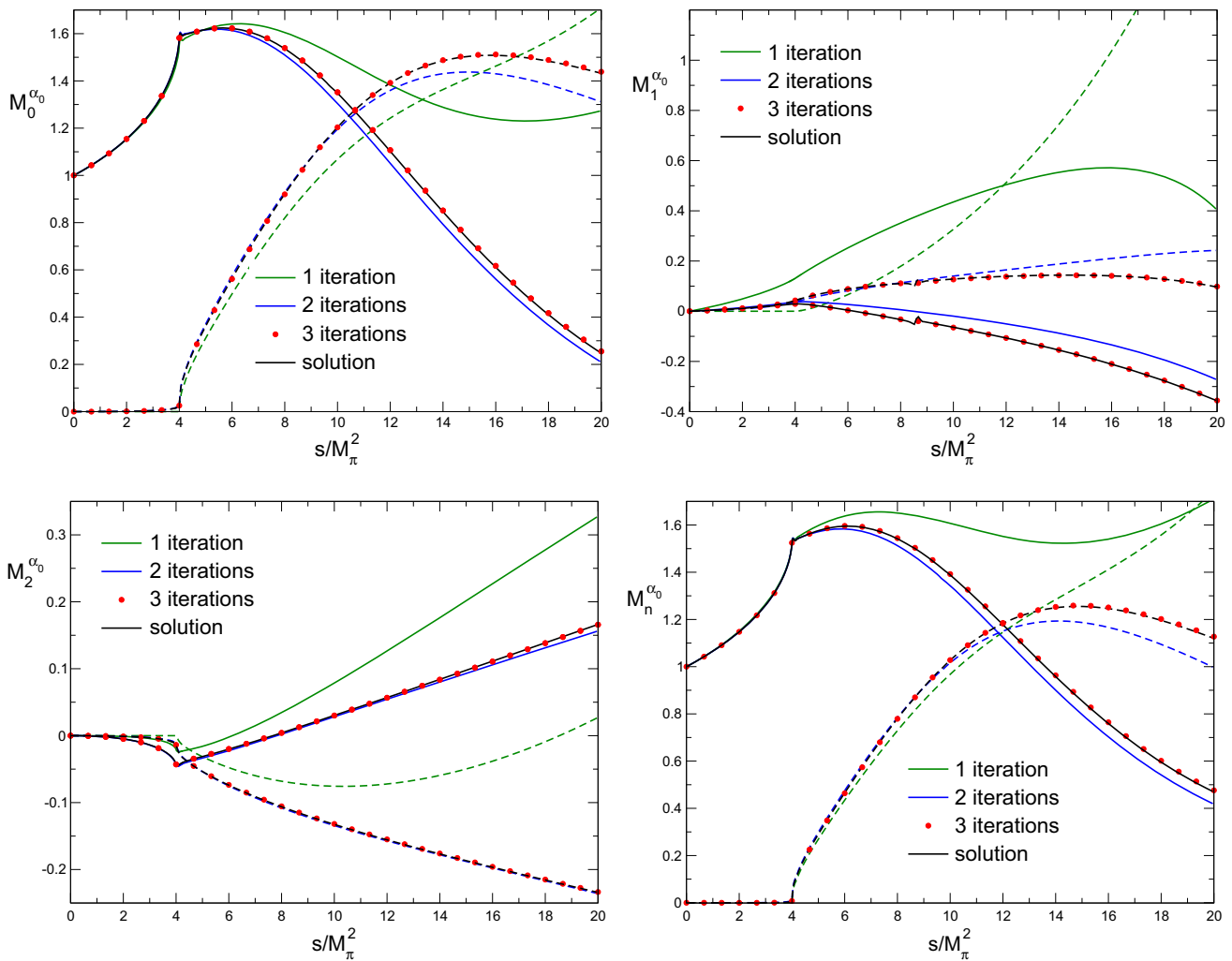
Fig. 2 Isospin components and neutral channel amplitude of the fundamental solution belonging to \alpha_0 (real and imaginary parts are shown as full and dashed lines, respectively). The plot illustrates the convergence
