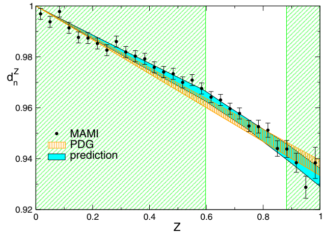
Fig. 16 Prediction obtained from the KLOE measurements of \eta \rightarrow \pi^+\pi^-\pi^0 [22] for the Z -distribution of the decay for \eta \rightarrow 3\pi^0 compared with the most recent MAMI results [25]. The shaded areas indicate the region where the cusps generated by the final state interaction do not show up
