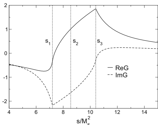
Fig. 23 Kernel relevant for the contributions from the horseshoe
