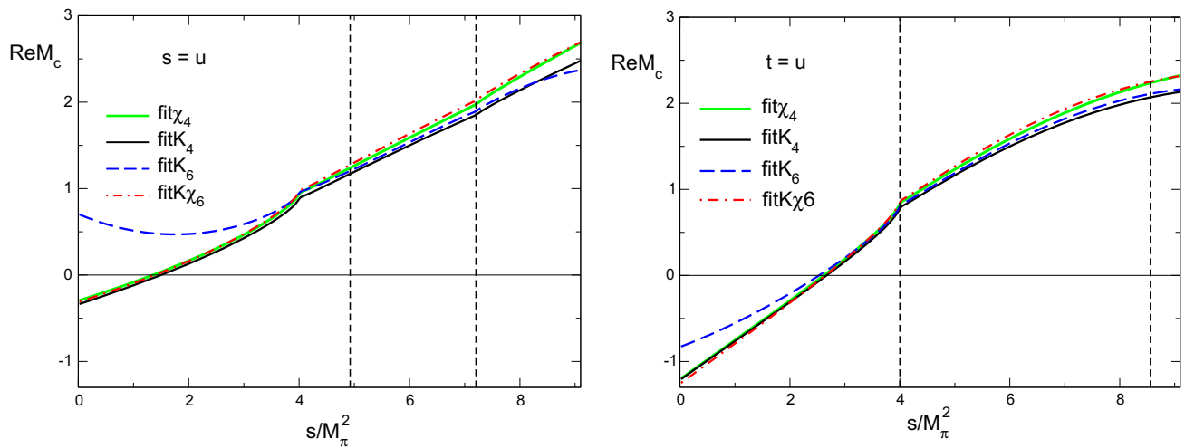
Fig. 10 Real parts of various dispersive solutions along the lines s = u and t = u
