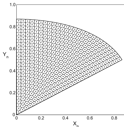
Fig. 24 Binning the physical region of the decay \eta \rightarrow 3\pi^0 . The bins are bounded by lines of constant \lambda and lines of constant \varphi . The dots mark their center of gravity
