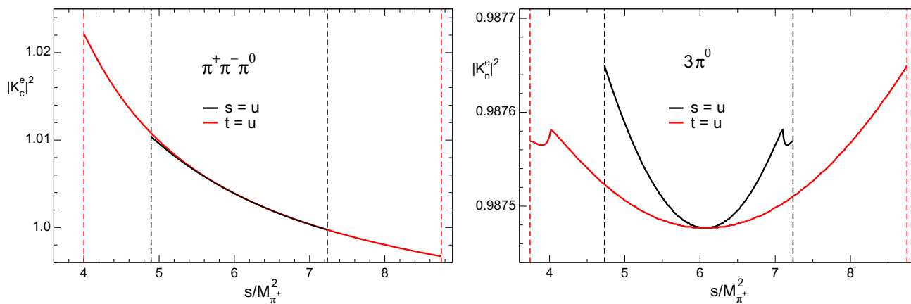
Fig. 7 One-loop representation: electromagnetic effects that are not accounted for in the self-energies of the particles. The plots show the square of the ratio between the full amplitude and what remains if the
