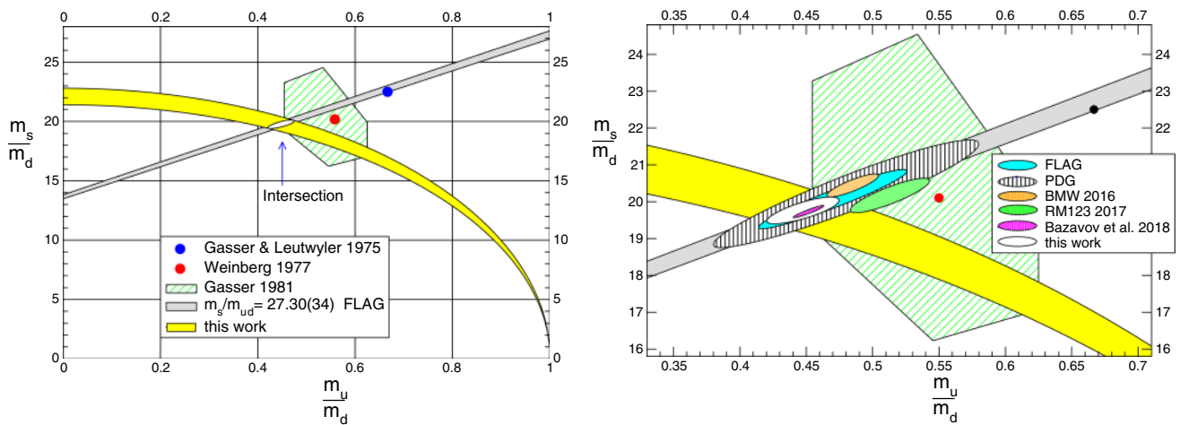
Fig. 21 Quark mass ratios (FLAG shown for N_f = 4 )
