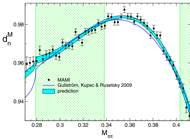
Fig. 17 Distribution in the variable M_{\pi\pi} = \sqrt{s} (GeV units). Prediction obtained from the KLOE measurements of \eta \rightarrow \pi^+\pi^-\pi^0 [22] compared with the MAMI results on \eta \rightarrow 3\pi^0 [25]. The shaded areas indicate the cusp-free regions
