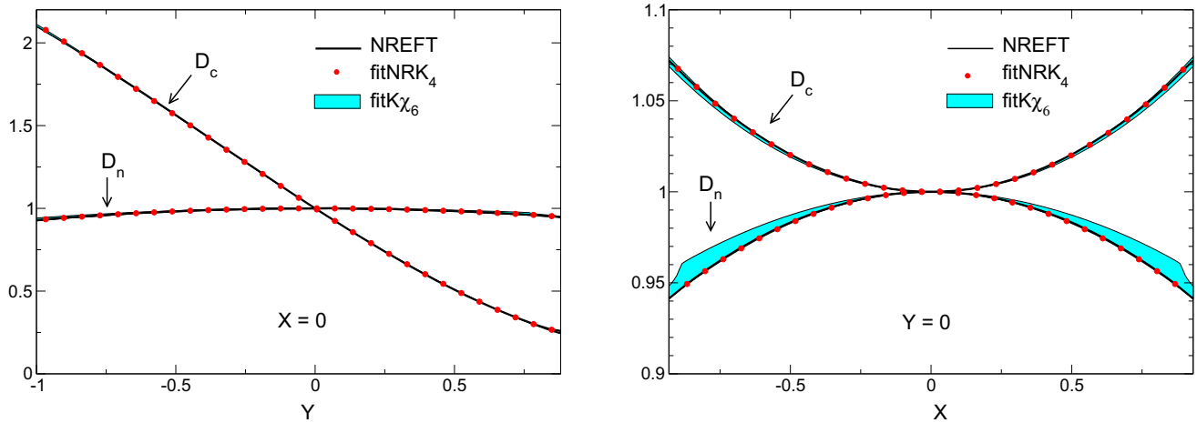
Fig. 12 Comparison of the nonrelativistic two-loop representation (black lines) with the dispersive solution that matches it (red dots): Dalitz plot distributions for the charged and neutral channels in the isospin limit. The uncertainty band belongs to our central solution,
