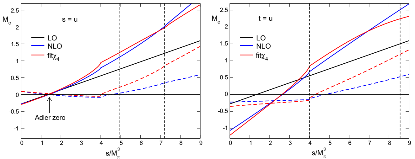
Fig. 4 Curvature generated by the final state interaction: comparison of the one loop representation with the dispersive solution that matches it at low energies. Real parts (full lines) and imaginary parts (dashed
