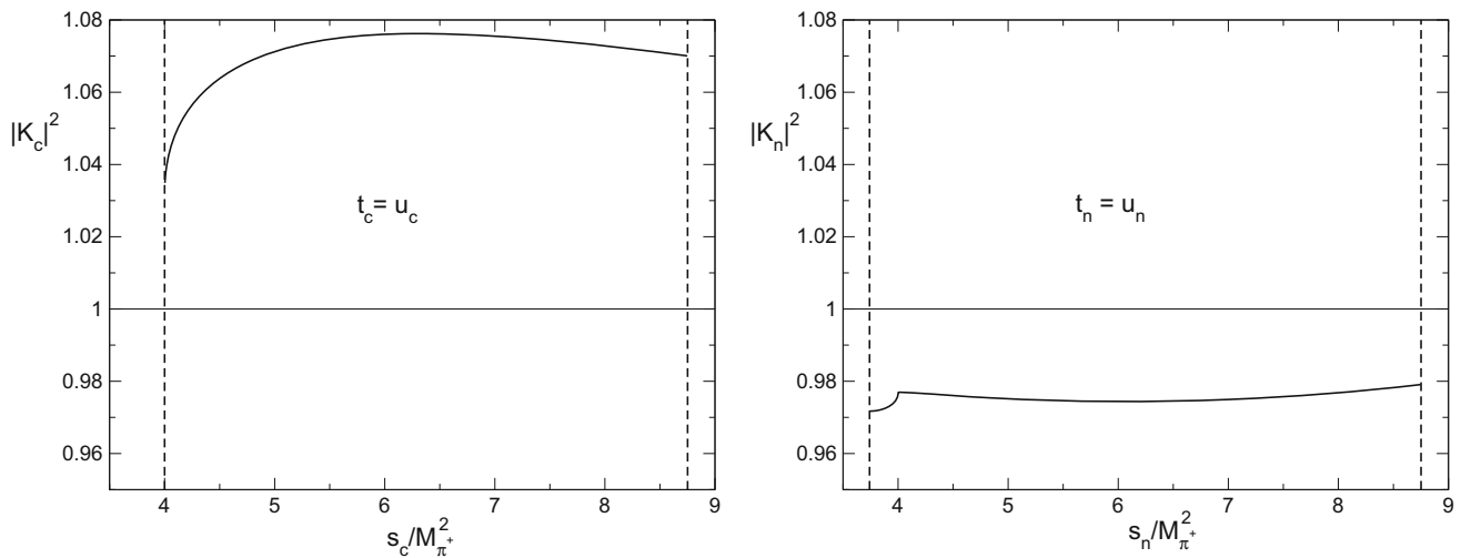
Fig. 8 One-loop representation: residual corrections in physical region
