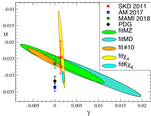
Fig. 19 Correlation between slope and curvature. The polynomial fits to the MAMI data for the decay \eta \rightarrow 3\pi^0 correspond to the large, slightly tilted ellipses in the left panel. They are compared with the results of Schneider, Kubis and Ditsche [42], Albaladejo and Mousalam [49], the A2 collaboration at MAMI [25] and the Particle Data Group [66]. The latter three neglect the curvature and are shown at \gamma = 0 . The matching solution \text{fit}\chi_4 , which exclusively relies on the-
