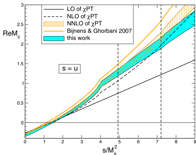
Fig. 14 Comparison of our result with the representations based on \chi PT at LO, NLO and NNLO (real part of the amplitude along the line s = u ). While the first two orders of the chiral perturbation series are parameter free, the NNLO representation does involve a set of low-energy constants that are not determined by the symmetry properties of the theory. The band labeled NNLO is obtained by determining these experimentally as outlined in Sect. 6.2
