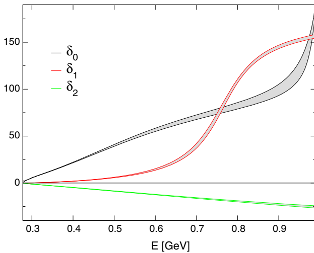
Fig. 1 Phase shifts of the leading \pi\pi partial waves
