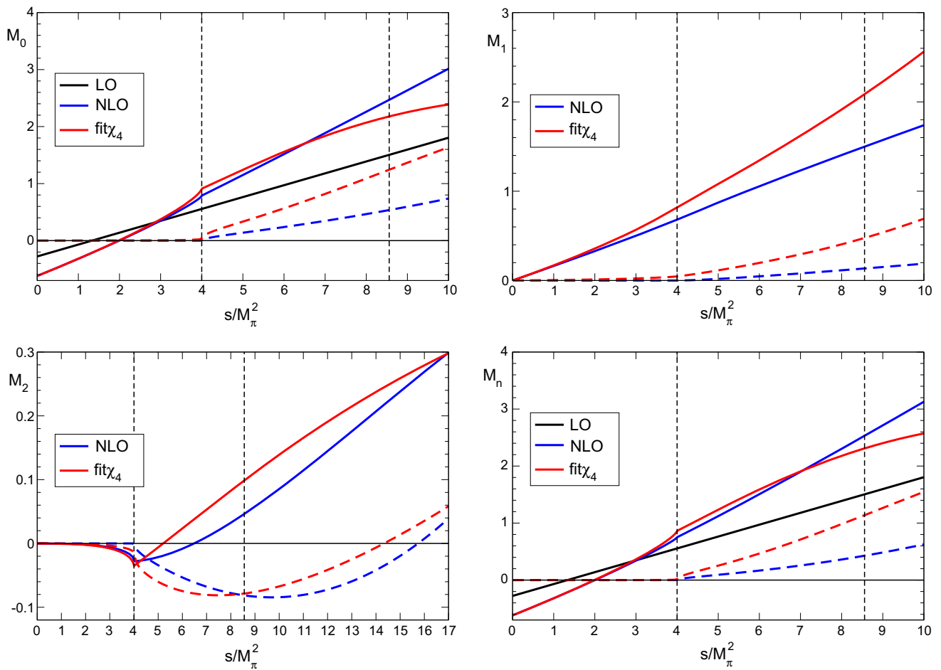
Fig. 3 Isospin components and neutral channel amplitude: comparison of the chiral representations to leading and first non-leading order with the dispersive solution that matches the NLO representation at small
