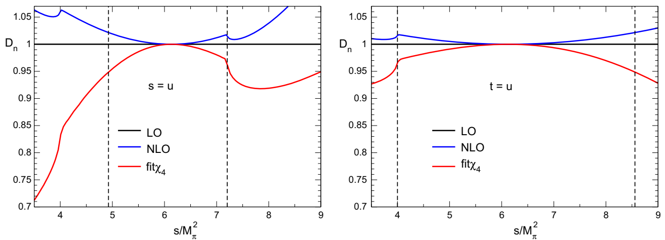
Fig. 5 Dalitz plot distribution (square of the amplitude normalized to 1 at the center) of the decay \eta \rightarrow 3\pi^0 , along the lines s = u and t = u . The plots show that accounting properly for the final state interaction changes the sign of the curvature and hence the sign of the slope \alpha
