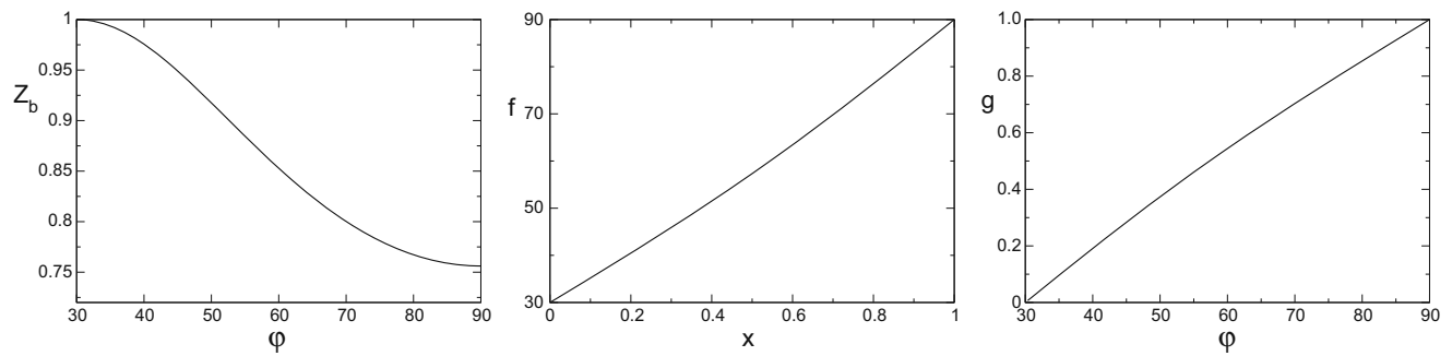
Fig. 25 Z_b(\varphi) describes the boundary of the physical region, f(\varphi) represents the fraction of the area spanned by the events in the interval \frac{\pi}{6} < \varphi' \leq \varphi . The plot of the inverse, g(x) , differs from the one for f(\varphi) only in the interchange of the horizontal and vertical axes
