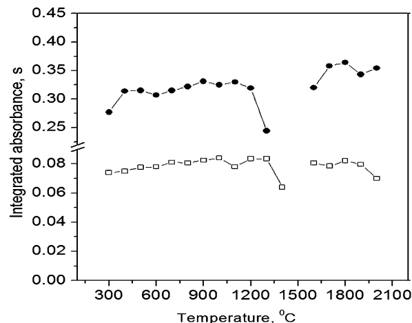
Fig. 1 Pyrolysis and atomization temperature curves for Ag in \text{CHCl}_3 extracts obtained from DLLME applied to (—●—) DOLT-3 and (—□—) 0.02 \mu\text{g L}^{-1} aqueous standard. Conditions: 5.0 mL of sample; 0.01% m/v DDTP; 500 \mu\text{L} acetone; 80 \mu\text{L} chloroform.
