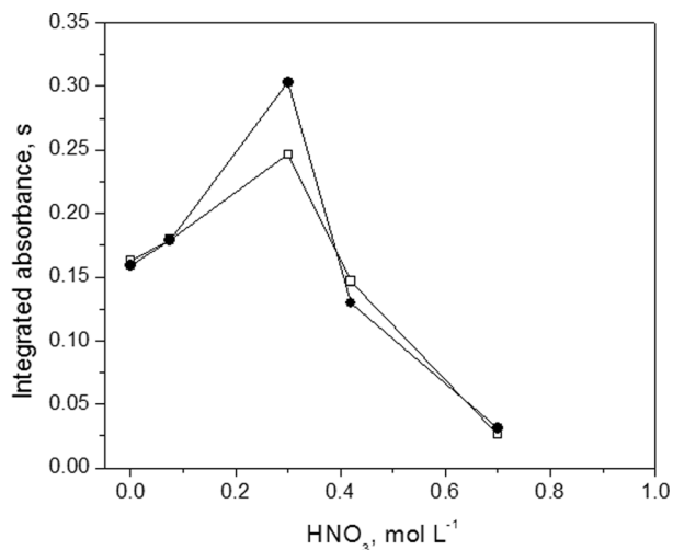
Fig. 2 Influence of HNO 3 concentration on the analytical signal for Ag obtained from DLLME applied to (—●—) DOLT-3 and a (—□—) 0.02 μg L -1 aqueous standard. Conditions: pyrolysis temperature 1100 °C; atomization temperature 1800 °C; 5.0 mL sample, 0.01% m/v DDTP; 500 μL acetone; 80 μL chloroform.
