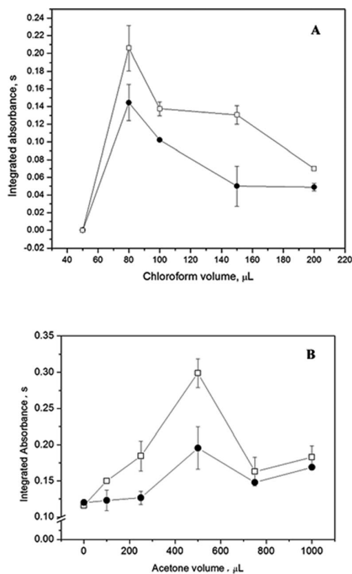
Fig. 3 (A) Effect of chloroform volume used for pre-concentration of Ag by DLLME using 500 μL acetone as dispersing solvent and (B) influence of acetone volume on the pre-concentration of Ag by DLLME using 80 μL chloroform as extractant. Legend: (—●—) DOLT-3 sample and (—□—) aqueous solution containing 0.02 μg L -1 Ag. Conditions: pyrolysis temperature 1100 °C; atomization temperature 1800 °C; 5.0 mL of sample, 0.01% m/v DDTP.
