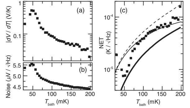
FIG. 5. Sensitivity and noise of temperature readout with quadrature detection. (a) Voltage responsivity at the output of the readout chain using heterodyne detection with f_{IF} = 1 MHz. Magnitude of the complex quantity is shown. (b) Mean spectral density of voltage noise in the frequency band from 10 kHz to 0.3 MHz. (c) Noise-equivalent temperature inferred from (a) and (b) including a \sqrt{2} gain from ideal homodyne detection (experiment, symbols) with superimposed theoretical models: Constant probing power in the small-signal regime (dashed line). Same with responsivity enhancement from explicit temperature dependence of I_c (thin solid line). Minimum achievable NET with optimized probing power at each temperature from a nonlinear model (thick line).
