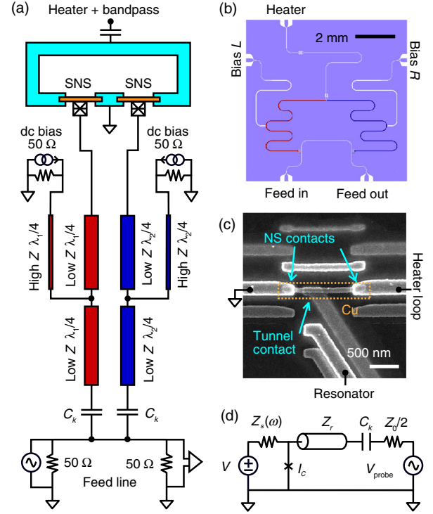
FIG. 1. The studied system. (a) Electrical schematic of the device and essential external components. The left and right halves of the device are functionally equivalent. Coplanar waveguides are used to define microwave resonance modes (at 4.688 and 5.668 GHz for blue and red elements in the illustration, respectively). The combination of low and high characteristic impedance (30 and 125 \Omega , respectively) sections of approximately \lambda/4 length allow dc biasing while increasing only slightly the losses of the microwave resonance. The resonators couple capacitively to a common feed line for frequency-multiplexed readout. The resonators terminate at small tunnel junctions between an Al electrode and a proximitized Al/Cu/Al (SNS) wire. The two SNS wires are part of the same superconducting loop [14] that couples electrical fluctuations from one wire to the other. Lastly, a microwave line is capacitively connected to a section of the loop and can be used to heat the SNS wires. Detailed wiring is shown in the Supplemental Material [15]. (b) Physical layout of device chip. The CPWs are fabricated from etched Nb on Si substrate. Bandpass filter for the heating line is implemented as an in-line half-wave resonator. (c) Scanning electron micrograph of one of the tunnel junctions fabricated with three-angle shadow evaporation. The disconnected copies of the mask pattern are a by-product of the fabrication method and do not affect the device characteristics. (d) Reduced circuit model used in theory. The dc shunt impedance Z_s(\omega = 0) is denoted by R_s .
