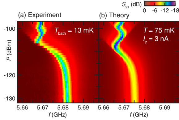
FIG. 4. Effect of large probe power on resonance line at zero bias. The experimental data (left) are obtained at the base temperature of the cryostat (13 mK). The theory data are calculated using a nonlinear model that describes the effect of large phase oscillations on effective junction dynamics. In the simulation, we use an artificially elevated constant temperature (75 mK) for the electromagnetic environment to suppress hysteresis in the model.
