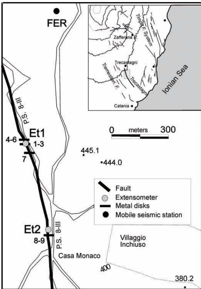
Figure 2. Location map of the extensometer stations Et1 and Et2, the discrete measurement sites, and the FER mobile seismic station.
