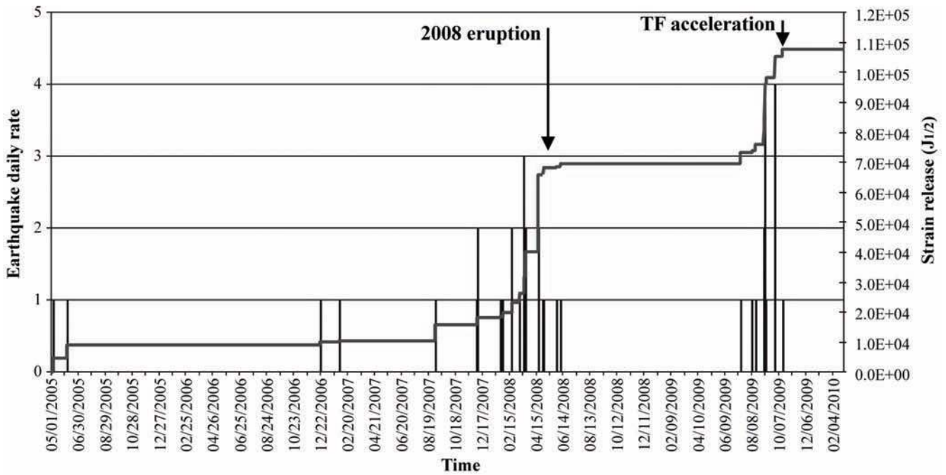
Figure 7. Earthquake daily rate and related strain release of the May 2005 to February 2010 seismicity that occurred in the narrow area reported in Figure 6D. The seismic strain release has been calculated as \sqrt{E} with the following relationship [Richter 1958]: \text{Log } E = 9.9 + 1.9 M_d - 0.024 M_d^2 , where M_d is the duration magnitude.
