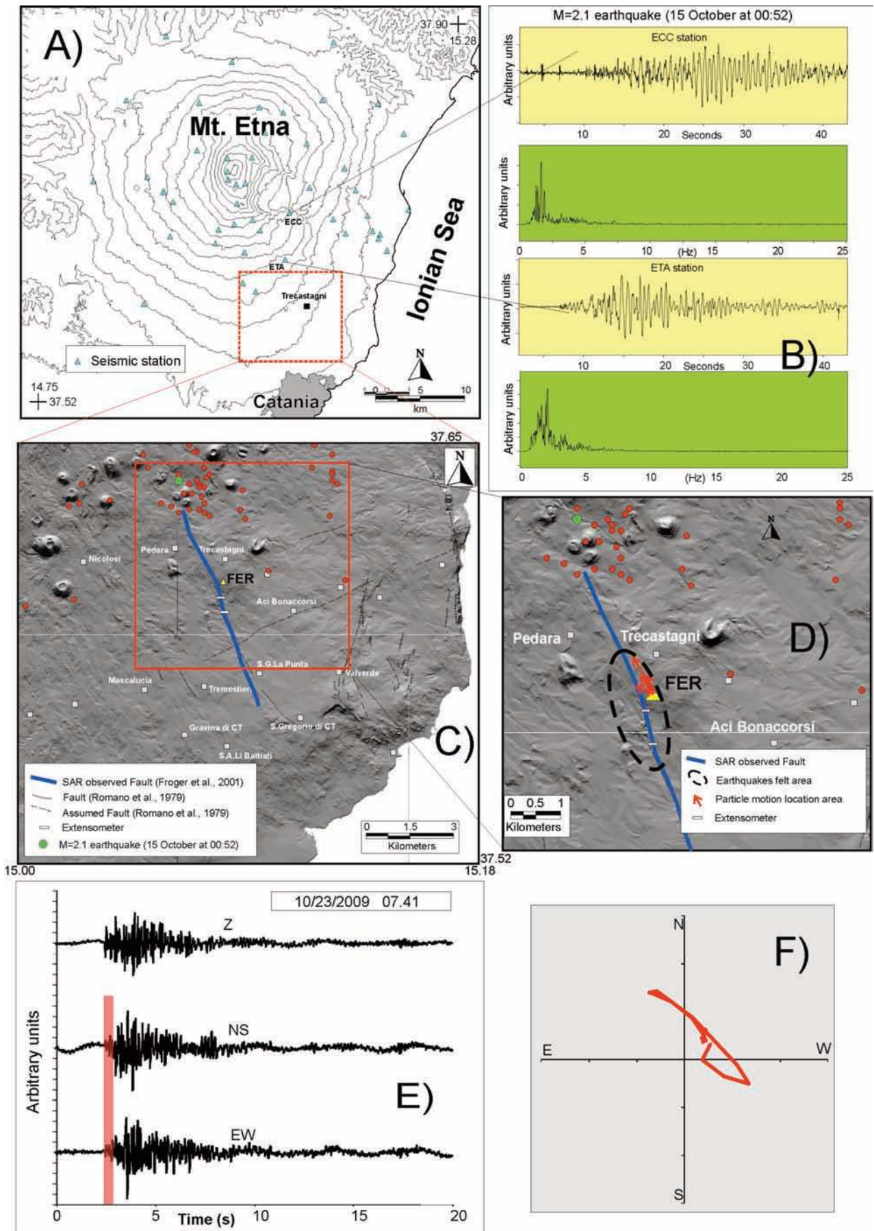
Figure 6. The Istituto Nazionale di Geofisica e Vulcanologia, Sezione di Catania, permanent seismic network (A; triangles), waveforms and spectra related to the October 15, 2009, 00:52 event recorded at the ECC (top panels) and ETA (lower panels) stations (B), seismicity recorded in the TF area between May 2005 and April 2010 (C, D), with microearthquake epicenters recorded at the FER station obtained from particle motion analysis and S-P seismic phase time lapse (D). Examples of waveform recorded at FER station (E); the red bar indicate the time window used for particle motion (F).
