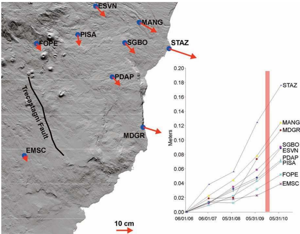
Figure 9. Global positioning system horizontal measurements between June 2006 and June 2010; arrows indicate the amplitude and direction of the displacements, and the graph shows the time series of the displacements. The red bar indicate the October 2009–January 2010 period.
