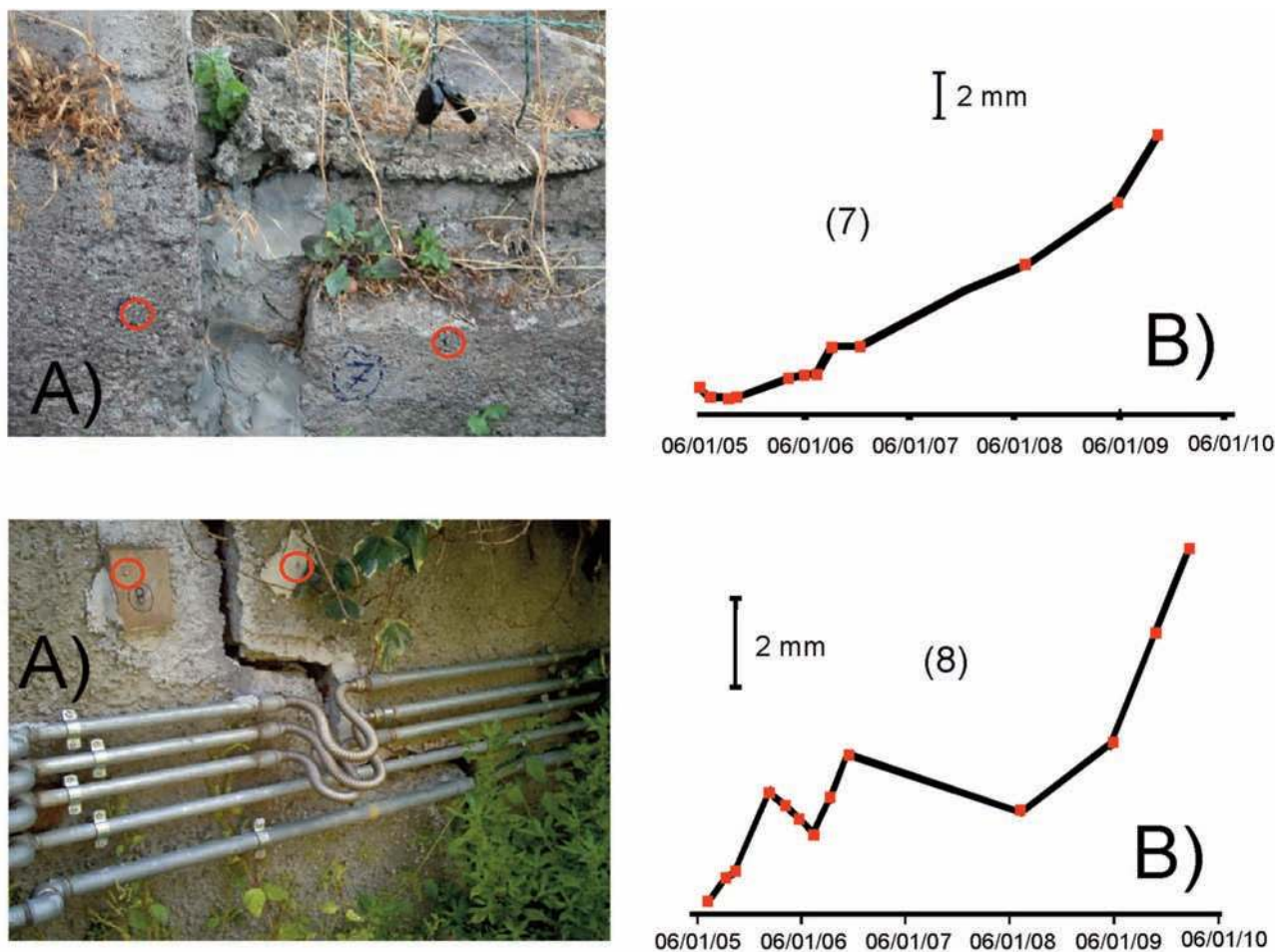
Figure 5. Photographs (A) and related data (B) of the n° 7 and n° 8 pairs of metal discs installed along the structure. Red circle evidence the metal discs. The graphs (B) indicates the changes in the distance between the metal discs.
