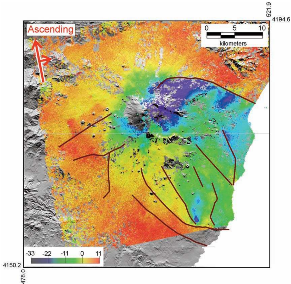
Figure 8. Mean ascending line-of-sight ground velocity (mm/yr) referring to the 2007 to 2009 time span. The map was obtained using the persistent scatterer software, known as StaMPS/MTI [Hooper 2008], using all of the available ENVISAT ascending data that was acquired for Mt. Etna from January 2007 to October 2009. The main discontinuities in the permanent scatterers velocity field detected by Bonforte et al. [2011] are shown as brown line. Red arrows indicate the trajectory (from South to North) of the satellite and its look direction toward East. The colour scale is in mm/year. The bottom left and top right corner coordinates are in km (WGS84 Datum, UTM projection, zone 33 north).
