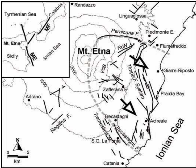
Figure 1. Surface-fault map of Mt. Etna. Inset: main regional fault systems: MF, Messina–Fiumefreddo line; ME, Malta Escarpment; RdN, Ripe della Naca; VdB, Valle del Bove. Gray line identifies the sliding sector.
